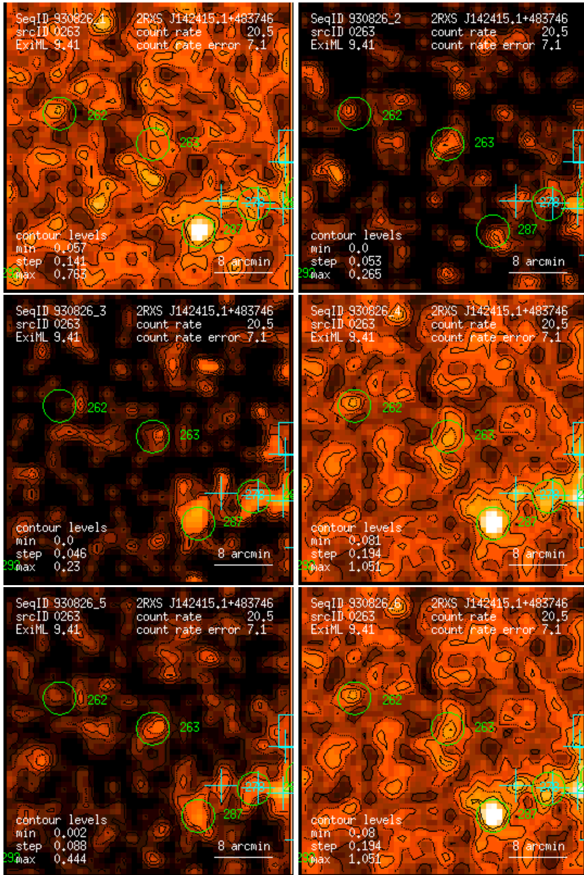
Figure 263: RASS 930826: detection 0263: band rate images, Gaussian filter: (1) PSPC channels 11 – 41, (2) 52 – 90, (3) 91 – 201, (4) 11 – 235, (5) 52 – 201, (6) 11 – 201. Broad band rates in counts/ks. Band rate contour levels in counts/ks/arcmin 2 .
