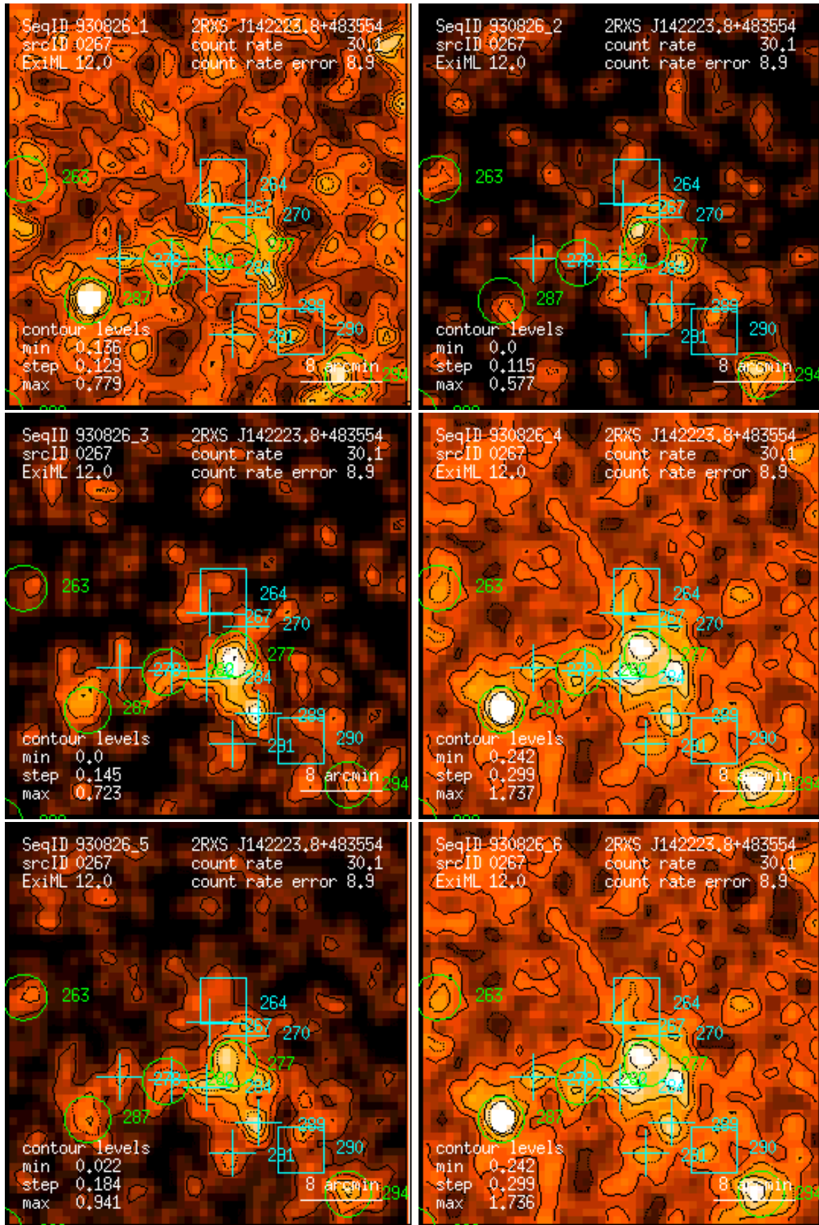
Figure 267: RASS 930826: detection 0267: band rate images, Gaussian filter: (1) PSPC channels 11 – 41, (2) 52 – 90, (3) 91 – 201, (4) 11 – 235, (5) 52 – 201, (6) 11 – 201. Broad band rates in counts/ks. Band rate contour levels in counts/ks/arcmin 2 .
