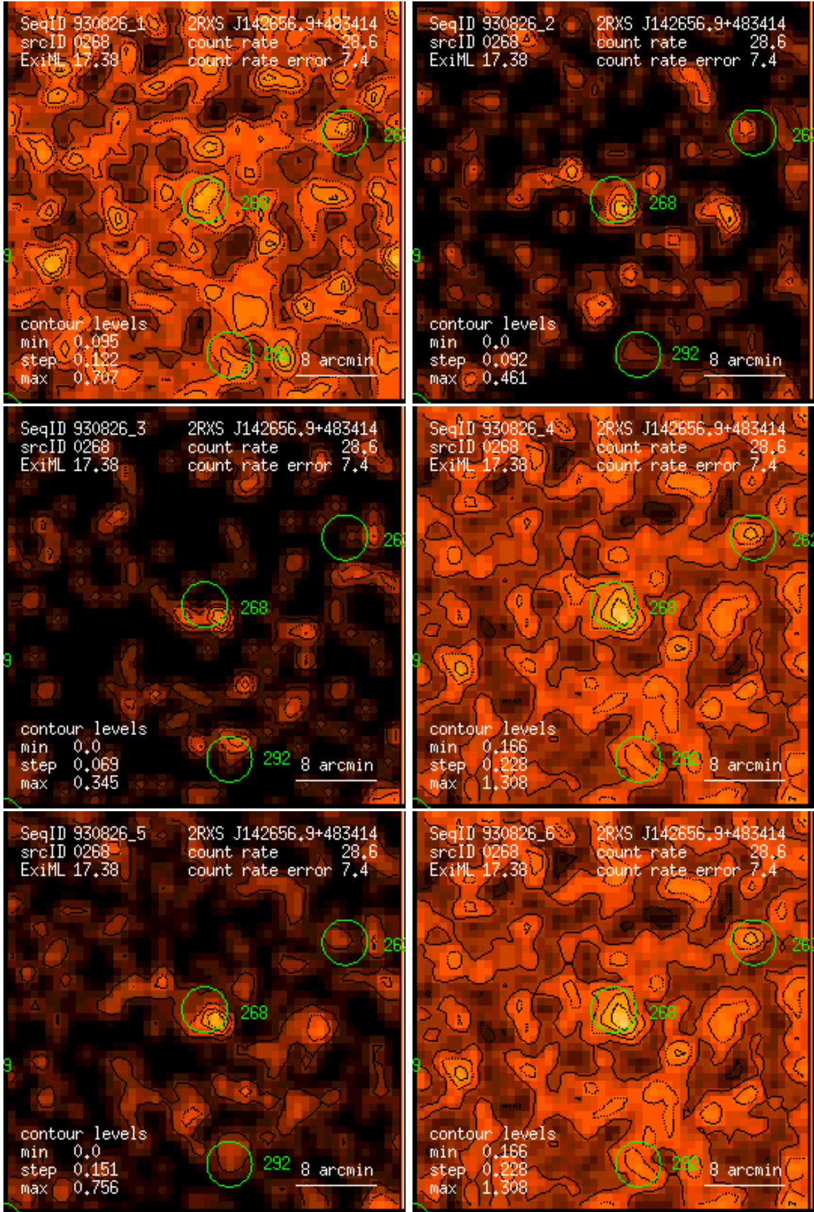
Figure 268: RASS 930826: detection 0268: band rate images, Gaussian filter: (1) PSPC channels 11 – 41, (2) 52 – 90, (3) 91 – 201, (4) 11 – 235, (5) 52 – 201, (6) 11 – 201. Broad band rates in counts/ks. Band rate contour levels in counts/ks/arcmin 2 .
