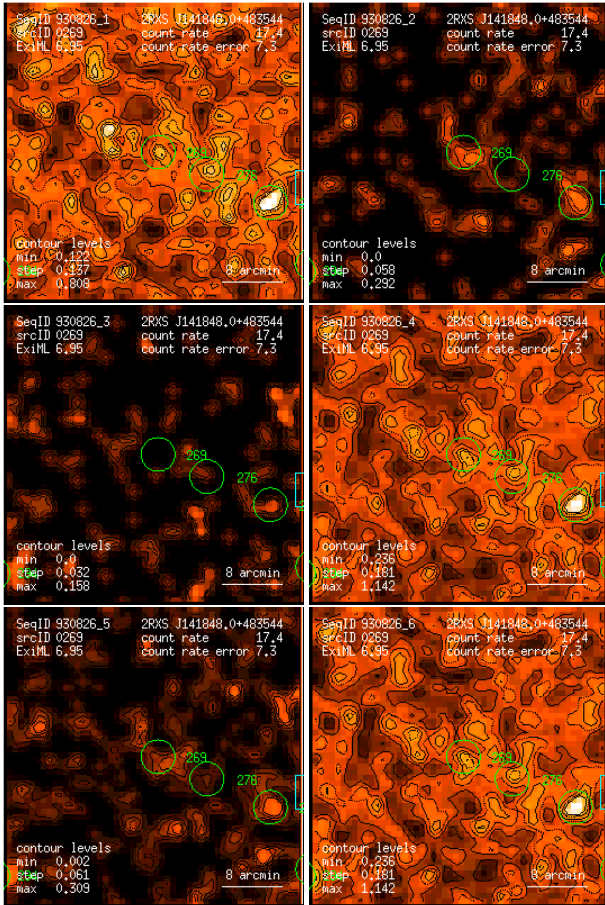
Figure 269: RASS 930826: detection 0269: band rate images, Gaussian filter: (1) PSPC channels 11 – 41, (2) 52 – 90, (3) 91 – 201, (4) 11 – 235, (5) 52 – 201, (6) 11 – 201. Broad band rates in counts/ks. Band rate contour levels in counts/ks/arcmin 2 .
