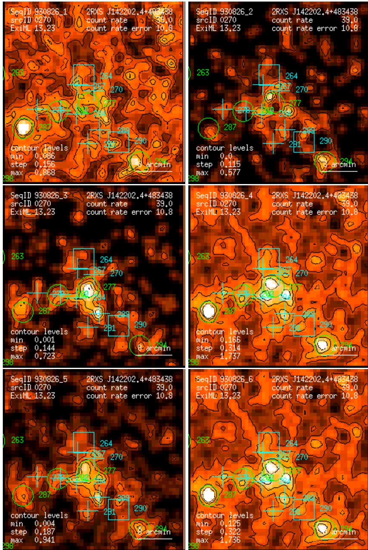
Figure 270: RASS 930826: detection 0270: band rate images, Gaussian filter: (1) PSPC channels 11 – 41, (2) 52 – 90, (3) 91 – 201, (4) 11 – 235, (5) 52 – 201, (6) 11 – 201. Broad band rates in counts/ks. Band rate contour levels in counts/ks/arcmin 2 .
