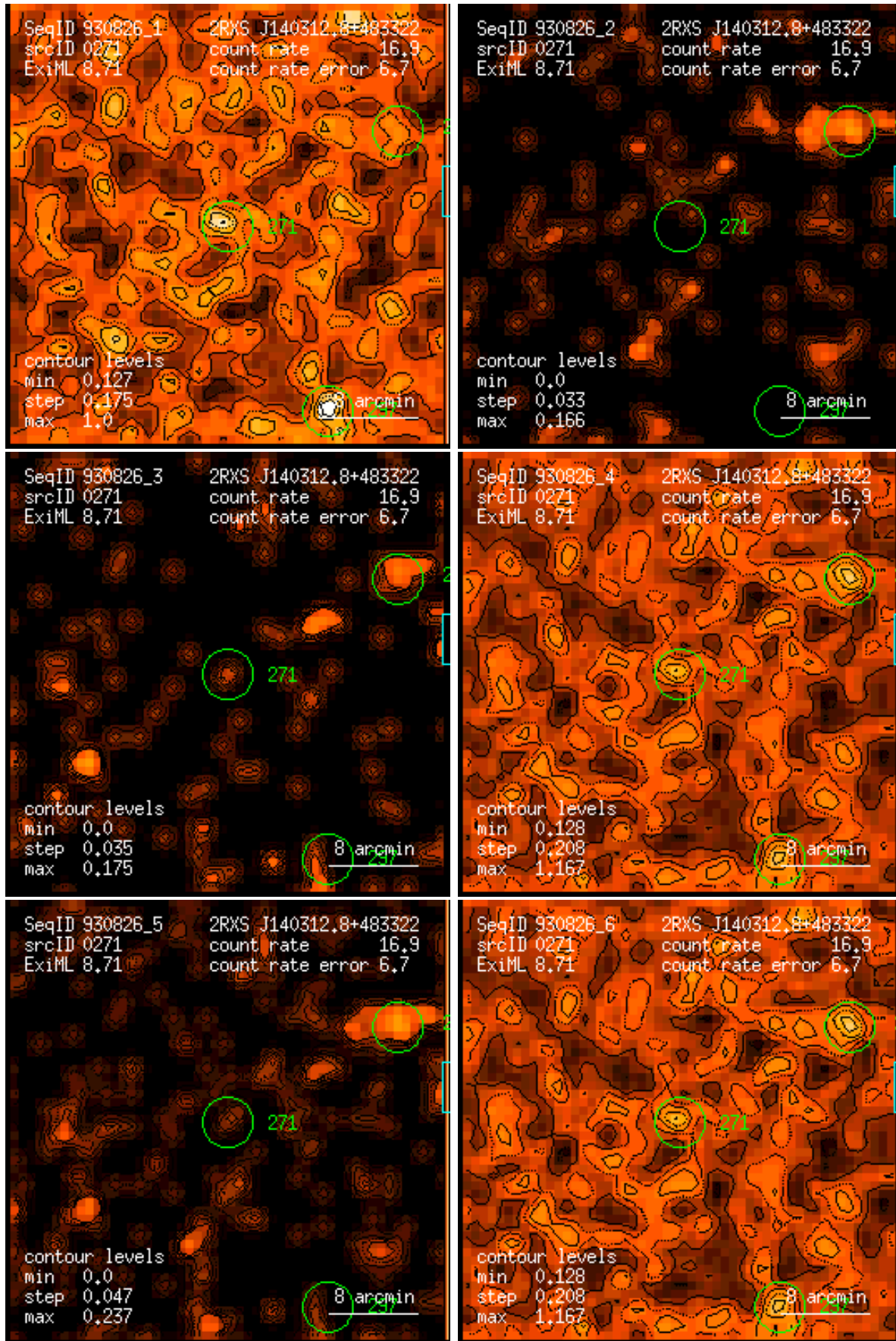
Figure 271: RASS 930826: detection 0271: band rate images, Gaussian filter: (1) PSPC channels 11 – 41, (2) 52 – 90, (3) 91 – 201, (4) 11 – 235, (5) 52 – 201, (6) 11 – 201. Broad band rates in counts/ks. Band rate contour levels in counts/ks/arcmin 2 .
