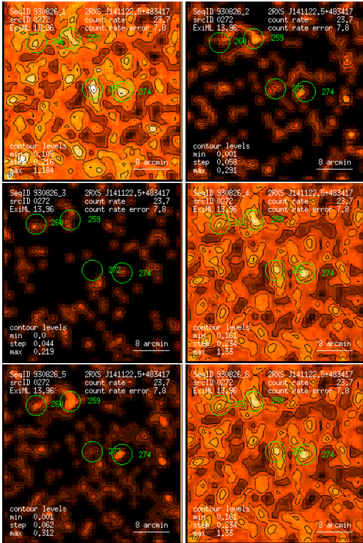
Figure 272: RASS 930826: detection 0272: band rate images, Gaussian filter: (1) PSPC channels 11 – 41, (2) 52 – 90, (3) 91 – 201, (4) 11 – 235, (5) 52 – 201, (6) 11 – 201. Broad band rates in counts/ks. Band rate contour levels in counts/ks/arcmin 2 .
