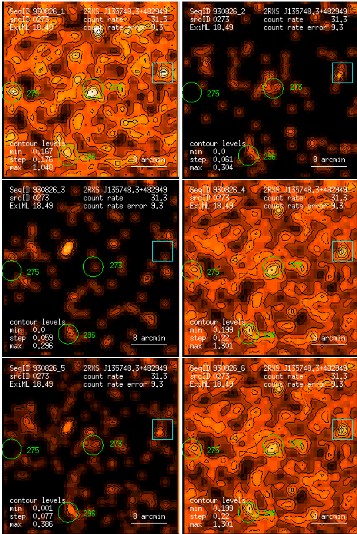
Figure 273: RASS 930826: detection 0273: band rate images, Gaussian filter: (1) PSPC channels 11 – 41, (2) 52 – 90, (3) 91 – 201, (4) 11 – 235, (5) 52 – 201, (6) 11 – 201. Broad band rates in counts/ks. Band rate contour levels in counts/ks/arcmin 2 .
