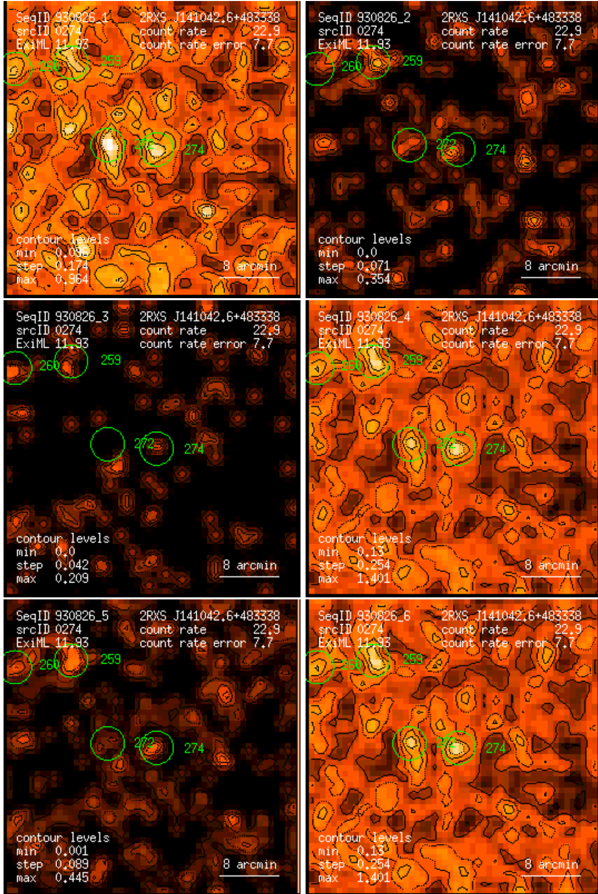
Figure 274: RASS 930826: detection 0274: band rate images, Gaussian filter: (1) PSPC channels 11 – 41, (2) 52 – 90, (3) 91 – 201, (4) 11 – 235, (5) 52 – 201, (6) 11 – 201. Broad band rates in counts/ks. Band rate contour levels in counts/ks/arcmin 2 .
