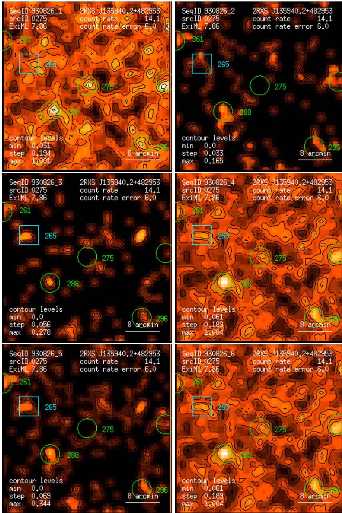
Figure 275: RASS 930826: detection 0275: band rate images, Gaussian filter: (1) PSPC channels 11 – 41, (2) 52 – 90, (3) 91 – 201, (4) 11 – 235, (5) 52 – 201, (6) 11 – 201. Broad band rates in counts/ks. Band rate contour levels in counts/ks/arcmin 2 .
