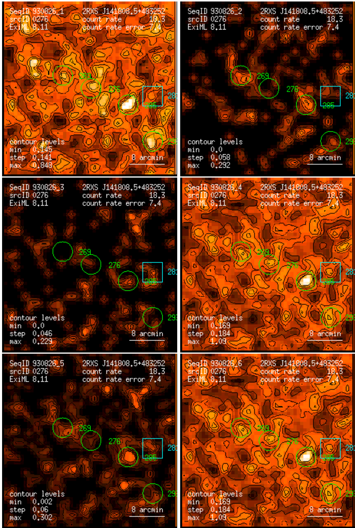
Figure 276: RASS 930826: detection 0276: band rate images, Gaussian filter: (1) PSPC channels 11 – 41, (2) 52 – 90, (3) 91 – 201, (4) 11 – 235, (5) 52 – 201, (6) 11 – 201. Broad band rates in counts/ks. Band rate contour levels in counts/ks/arcmin 2 .
