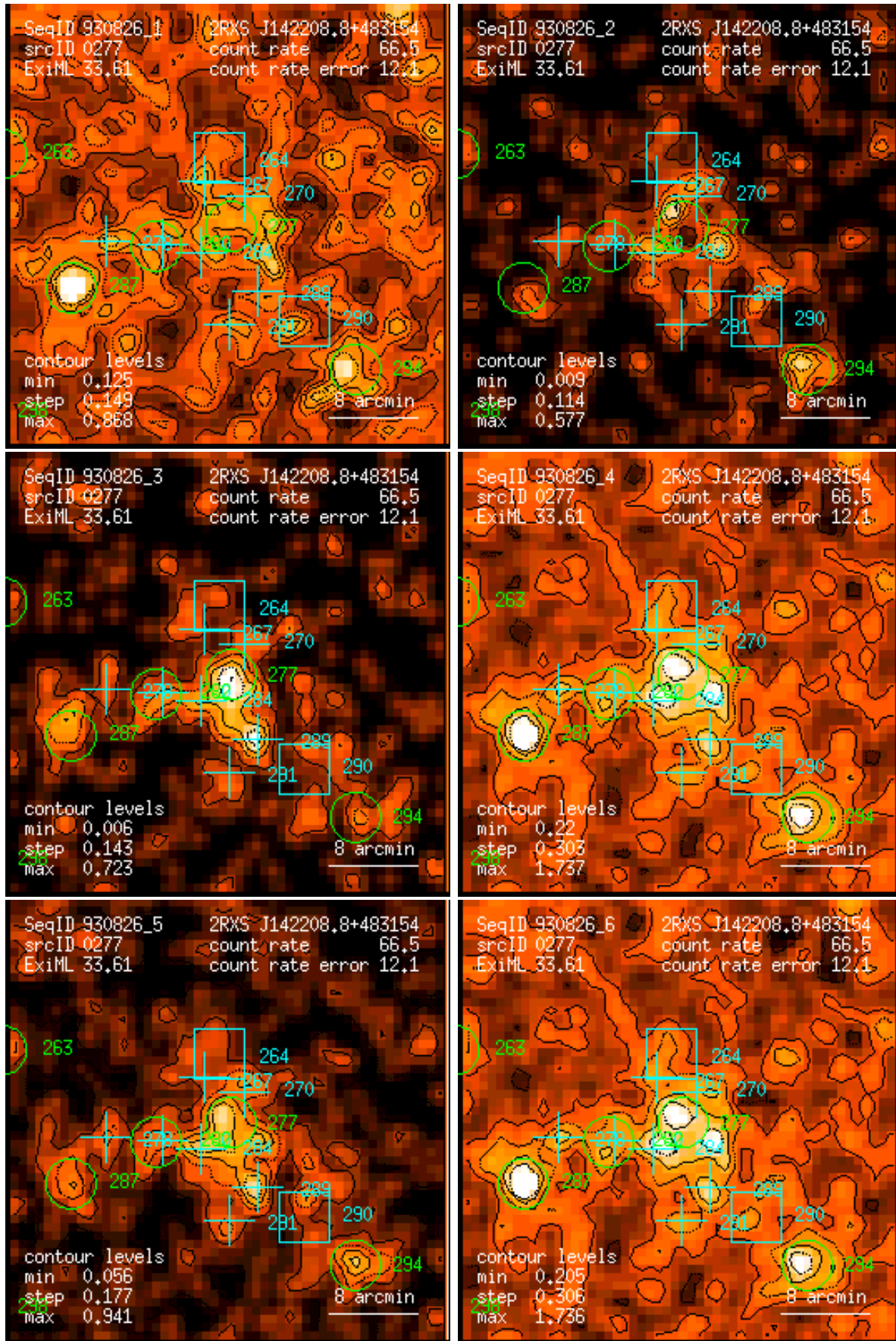
Figure 277: RASS 930826: detection 0277: band rate images, Gaussian filter: (1) PSPC channels 11 – 41, (2) 52 – 90, (3) 91 – 201, (4) 11 – 235, (5) 52 – 201, (6) 11 – 201. Broad band rates in counts/ks. Band rate contour levels in counts/ks/arcmin 2 .
