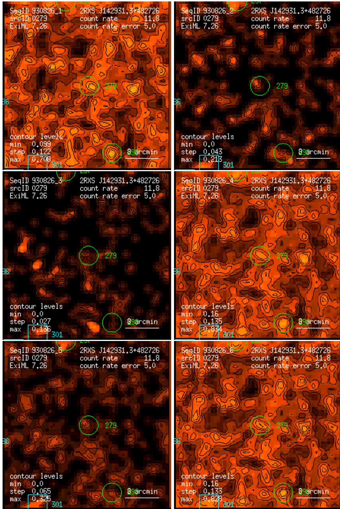
Figure 279: RASS 930826: detection 0279: band rate images, Gaussian filter: (1) PSPC channels 11 – 41, (2) 52 – 90, (3) 91 – 201, (4) 11 – 235, (5) 52 – 201, (6) 11 – 201. Broad band rates in counts/ks. Band rate contour levels in counts/ks/arcmin 2 .
