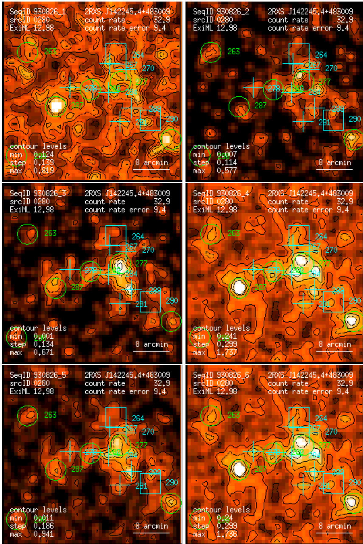
Figure 280: RASS 930826: detection 0280: band rate images, Gaussian filter: (1) PSPC channels 11 – 41, (2) 52 – 90, (3) 91 – 201, (4) 11 – 235, (5) 52 – 201, (6) 11 – 201. Broad band rates in counts/ks. Band rate contour levels in counts/ks/arcmin 2 .
