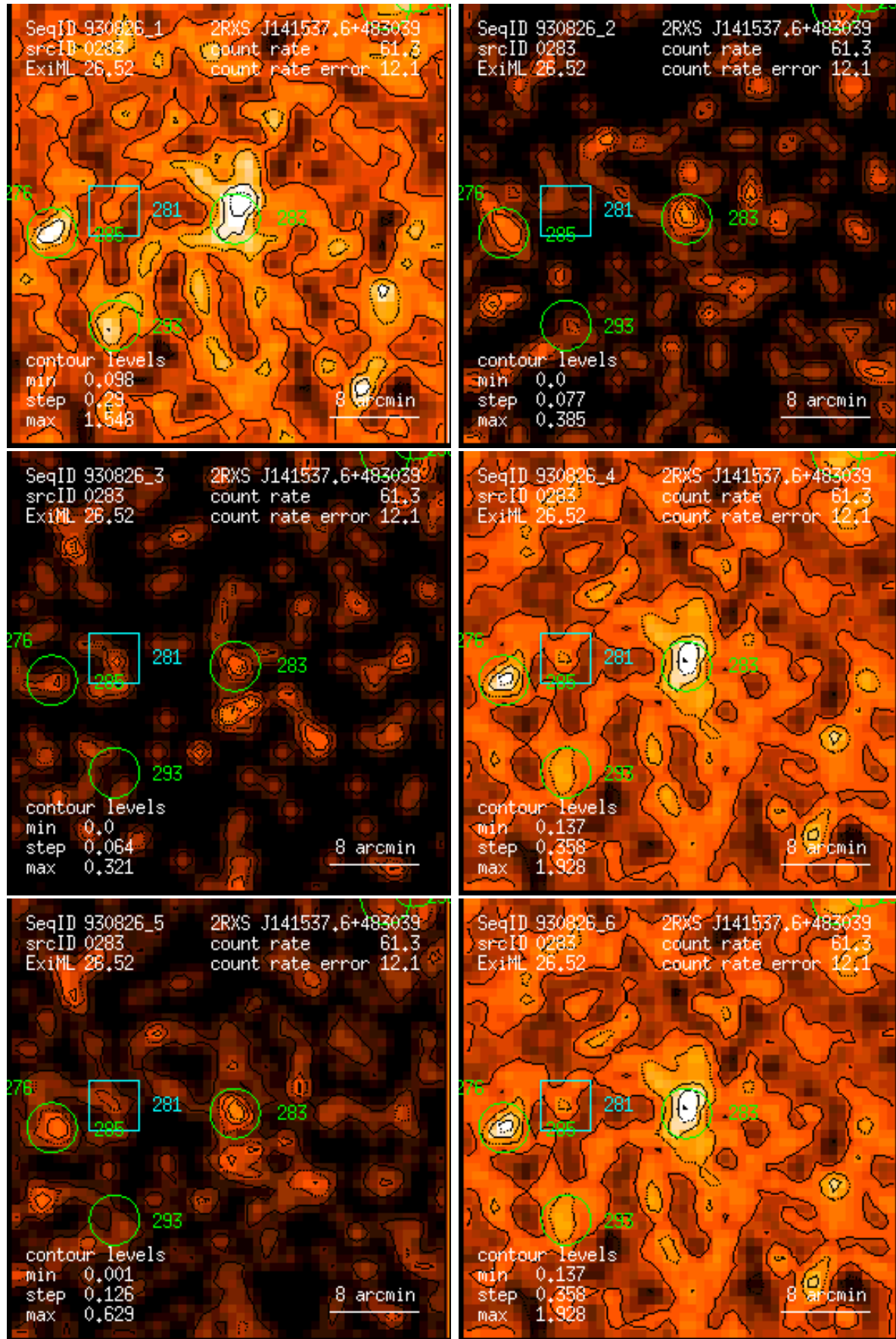
Figure 283: RASS 930826: detection 0283: band rate images, Gaussian filter: (1) PSPC channels 11 – 41, (2) 52 – 90, (3) 91 – 201, (4) 11 – 235, (5) 52 – 201, (6) 11 – 201. Broad band rates in counts/ks. Band rate contour levels in counts/ks/arcmin 2 .
