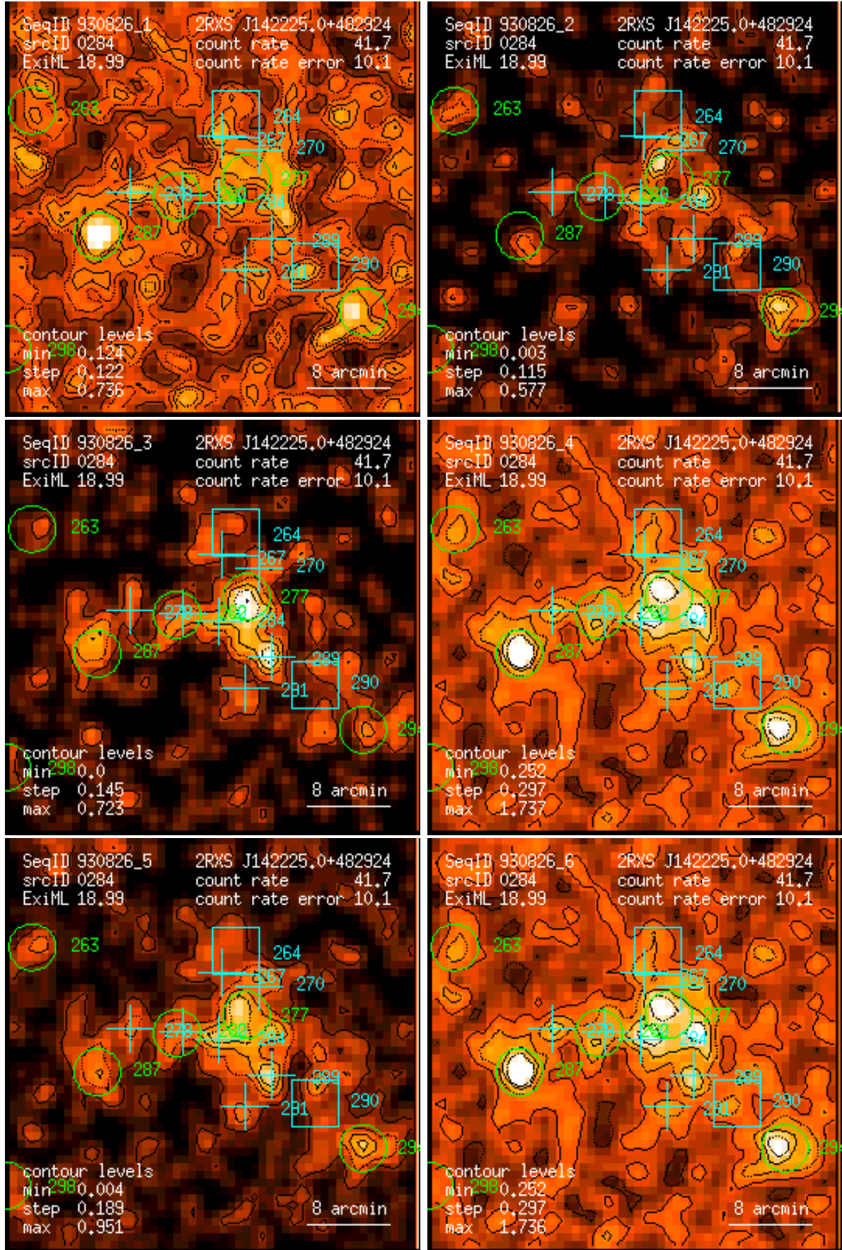
Figure 284: RASS 930826: detection 0284: band rate images, Gaussian filter: (1) PSPC channels 11 – 41, (2) 52 – 90, (3) 91 – 201, (4) 11 – 235, (5) 52 – 201, (6) 11 – 201. Broad band rates in counts/ks. Band rate contour levels in counts/ks/arcmin 2 .
