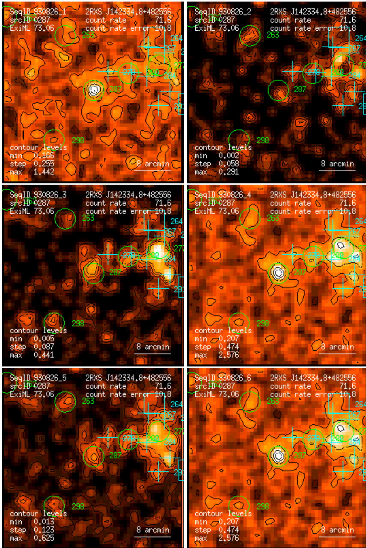
Figure 287: RASS 930826: detection 0287: band rate images, Gaussian filter: (1) PSPC channels 11 – 41, (2) 52 – 90, (3) 91 – 201, (4) 11 – 235, (5) 52 – 201, (6) 11 – 201. Broad band rates in counts/ks. Band rate contour levels in counts/ks/arcmin 2 .
