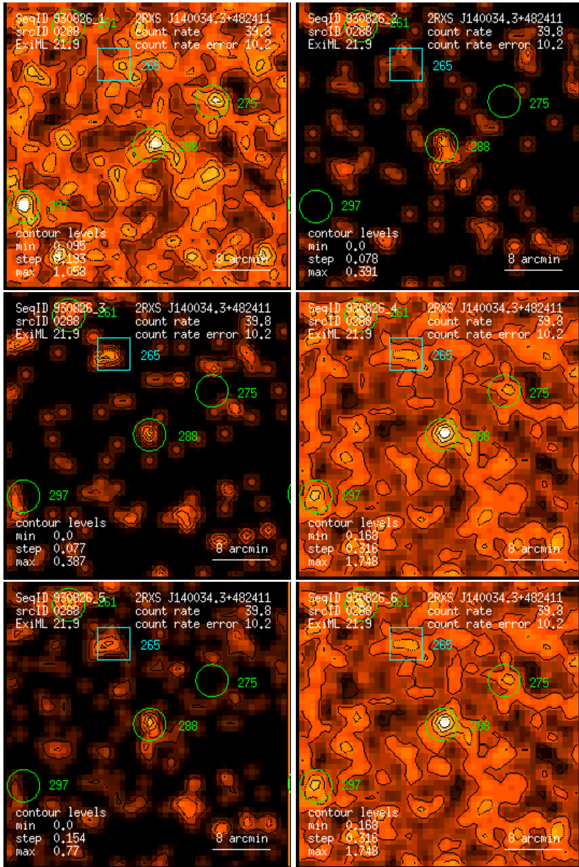
Figure 288: RASS 930826: detection 0288: band rate images, Gaussian filter: (1) PSPC channels 11 – 41, (2) 52 – 90, (3) 91 – 201, (4) 11 – 235, (5) 52 – 201, (6) 11 – 201. Broad band rates in counts/ks. Band rate contour levels in counts/ks/arcmin 2 .
