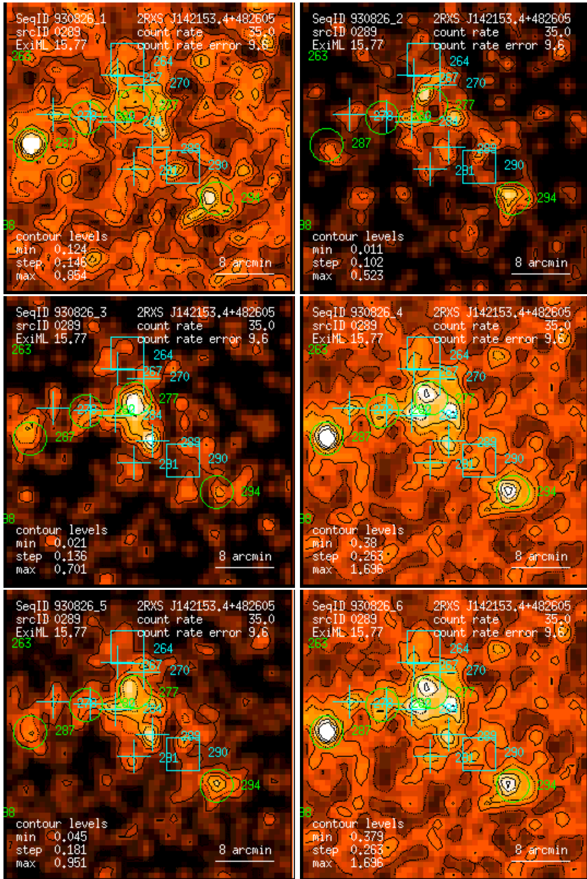
Figure 289: RASS 930826: detection 0289: band rate images, Gaussian filter: (1) PSPC channels 11 – 41, (2) 52 – 90, (3) 91 – 201, (4) 11 – 235, (5) 52 – 201, (6) 11 – 201. Broad band rates in counts/ks. Band rate contour levels in counts/ks/arcmin 2 .
