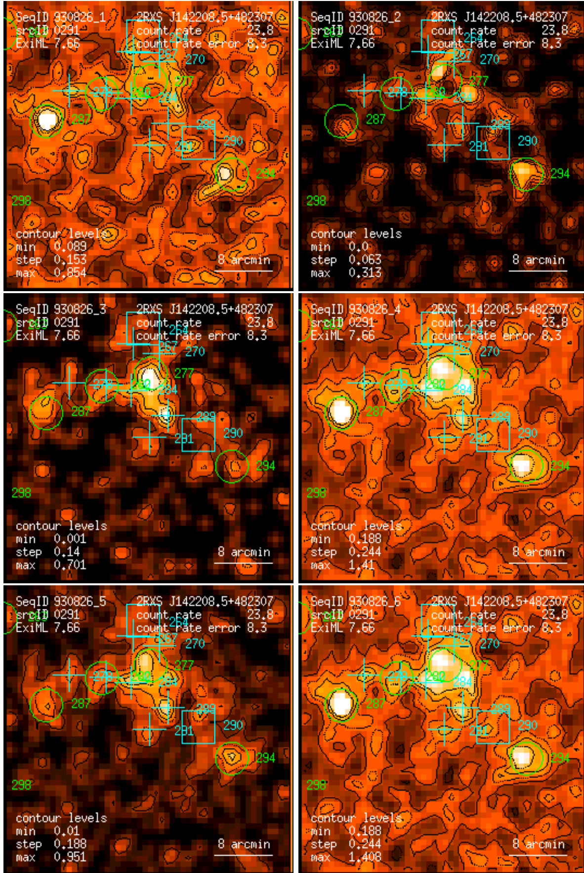
Figure 291: RASS 930826: detection 0291: band rate images, Gaussian filter: (1) PSPC channels 11 – 41, (2) 52 – 90, (3) 91 – 201, (4) 11 – 235, (5) 52 – 201, (6) 11 – 201. Broad band rates in counts/ks. Band rate contour levels in counts/ks/arcmin 2 .
