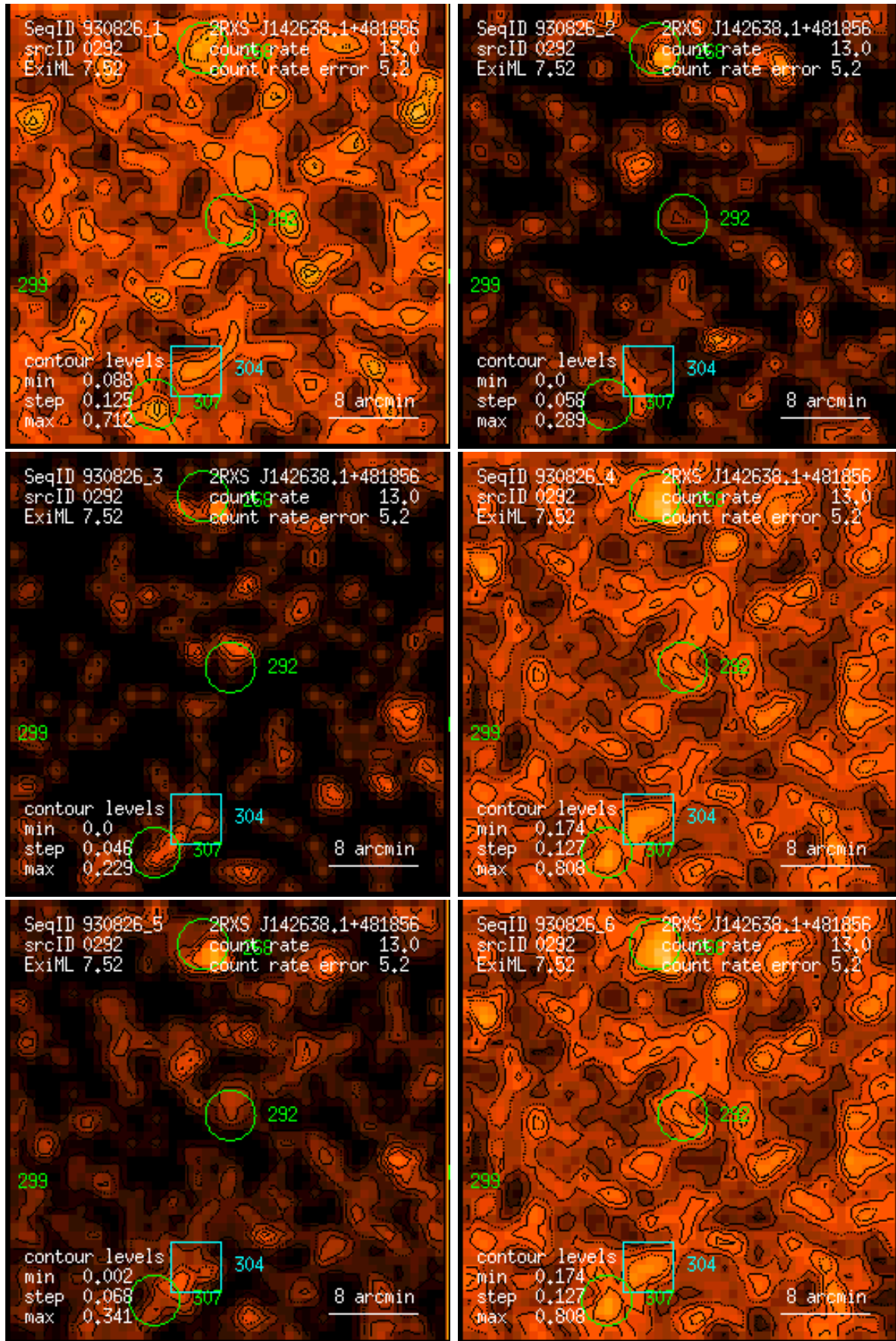
Figure 292: RASS 930826: detection 0292: band rate images, Gaussian filter: (1) PSPC channels 11 – 41, (2) 52 – 90, (3) 91 – 201, (4) 11 – 235, (5) 52 – 201, (6) 11 – 201. Broad band rates in counts/ks. Band rate contour levels in counts/ks/arcmin 2 .
