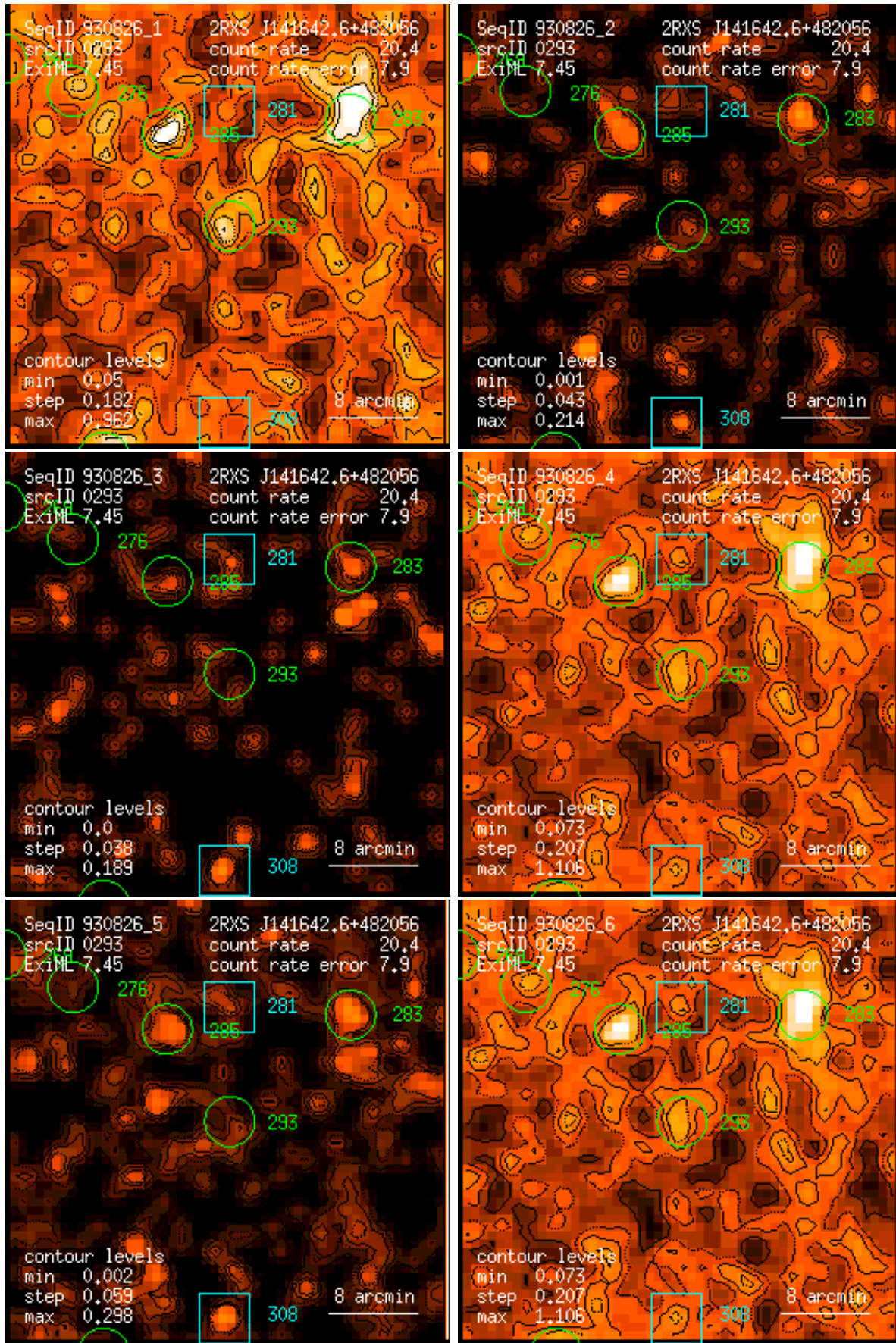
Figure 293: RASS 930826: detection 0293: band rate images, Gaussian filter: (1) PSPC channels 11 – 41, (2) 52 – 90, (3) 91 – 201, (4) 11 – 235, (5) 52 – 201, (6) 11 – 201. Broad band rates in counts/ks. Band rate contour levels in counts/ks/arcmin 2 .
