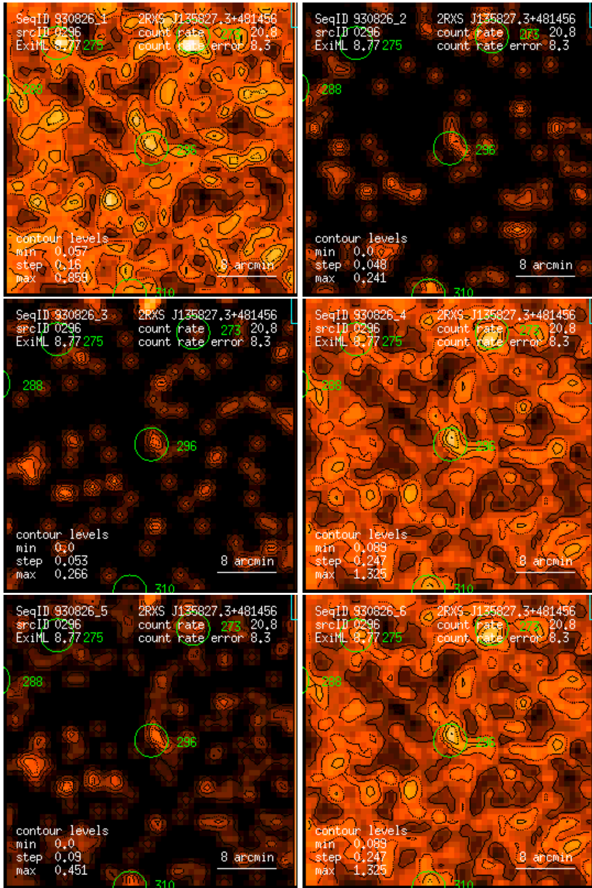
Figure 296: RASS 930826: detection 0296: band rate images, Gaussian filter: (1) PSPC channels 11 – 41, (2) 52 – 90, (3) 91 – 201, (4) 11 – 235, (5) 52 – 201, (6) 11 – 201. Broad band rates in counts/ks. Band rate contour levels in counts/ks/arcmin 2 .
