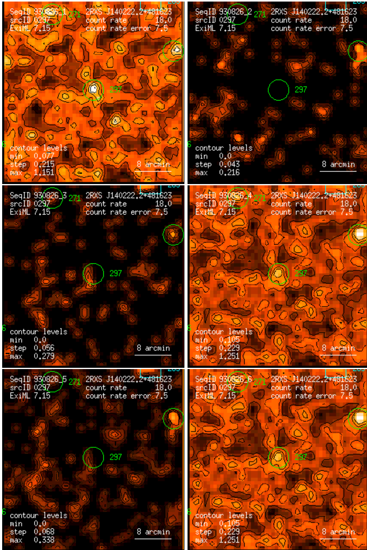
Figure 297: RASS 930826: detection 0297: band rate images, Gaussian filter: (1) PSPC channels 11 – 41, (2) 52 – 90, (3) 91 – 201, (4) 11 – 235, (5) 52 – 201, (6) 11 – 201. Broad band rates in counts/ks. Band rate contour levels in counts/ks/arcmin 2 .
