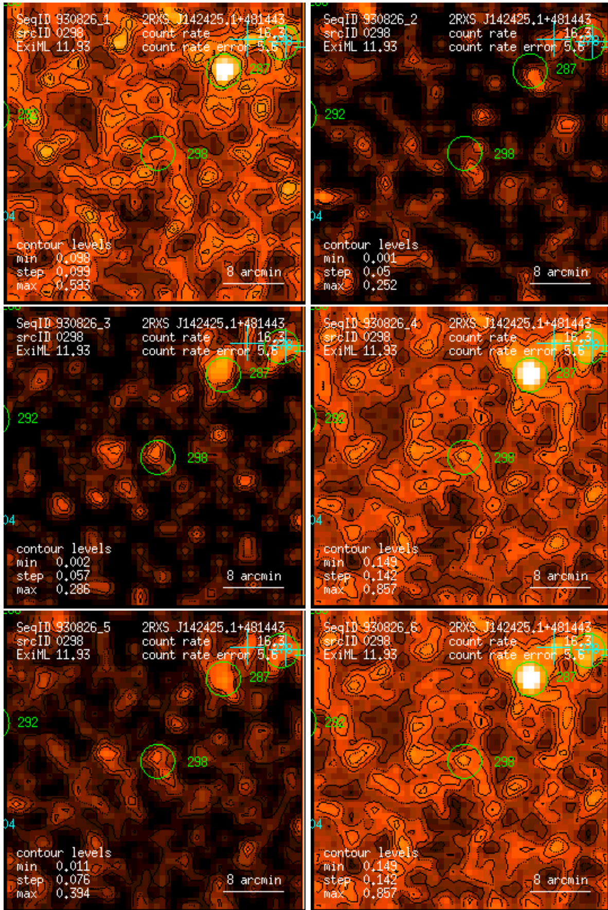
Figure 298: RASS 930826: detection 0298: band rate images, Gaussian filter: (1) PSPC channels 11 – 41, (2) 52 – 90, (3) 91 – 201, (4) 11 – 235, (5) 52 – 201, (6) 11 – 201. Broad band rates in counts/ks. Band rate contour levels in counts/ks/arcmin 2 .
