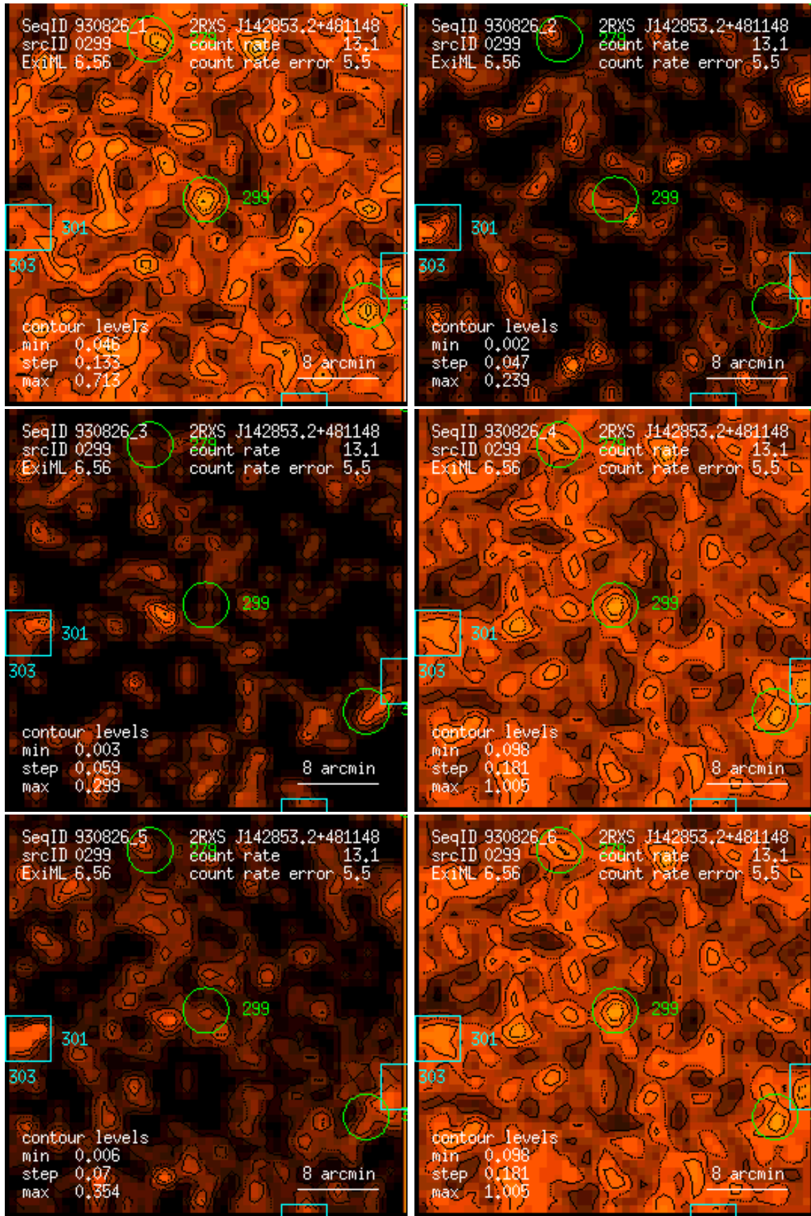
Figure 299: RASS 930826: detection 0299: band rate images, Gaussian filter: (1) PSPC channels 11 – 41, (2) 52 – 90, (3) 91 – 201, (4) 11 – 235, (5) 52 – 201, (6) 11 – 201. Broad band rates in counts/ks. Band rate contour levels in counts/ks/arcmin 2 .
