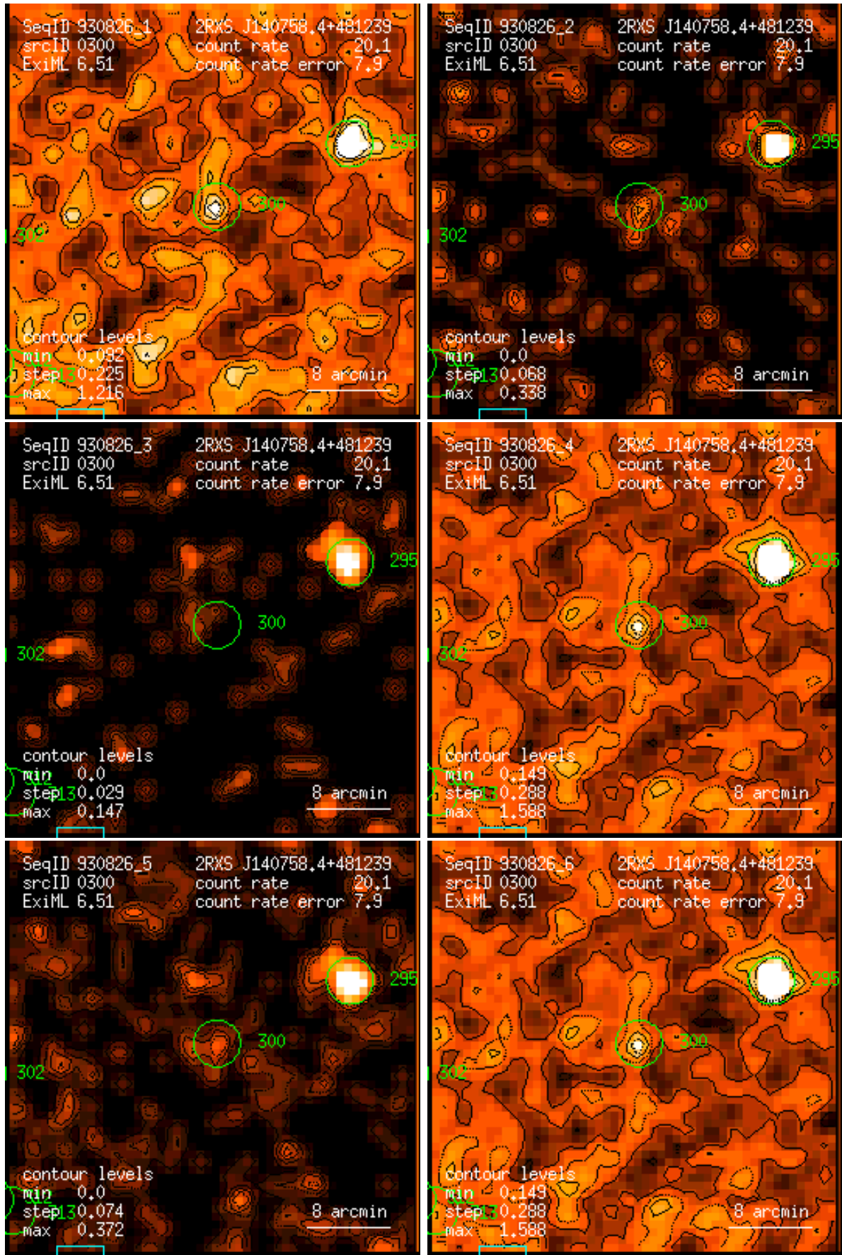
Figure 300: RASS 930826: detection 0300: band rate images, Gaussian filter: (1) PSPC channels 11 – 41, (2) 52 – 90, (3) 91 – 201, (4) 11 – 235, (5) 52 – 201, (6) 11 – 201. Broad band rates in counts/ks. Band rate contour levels in counts/ks/arcmin 2 .
