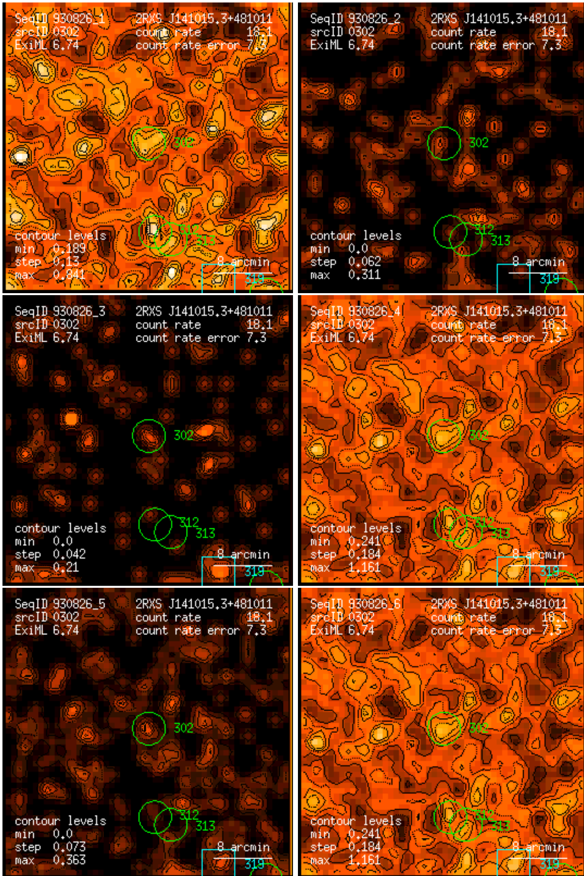
Figure 302: RASS 930826: detection 0302: band rate images, Gaussian filter: (1) PSPC channels 11 – 41, (2) 52 – 90, (3) 91 – 201, (4) 11 – 235, (5) 52 – 201, (6) 11 – 201. Broad band rates in counts/ks. Band rate contour levels in counts/ks/arcmin 2 .
