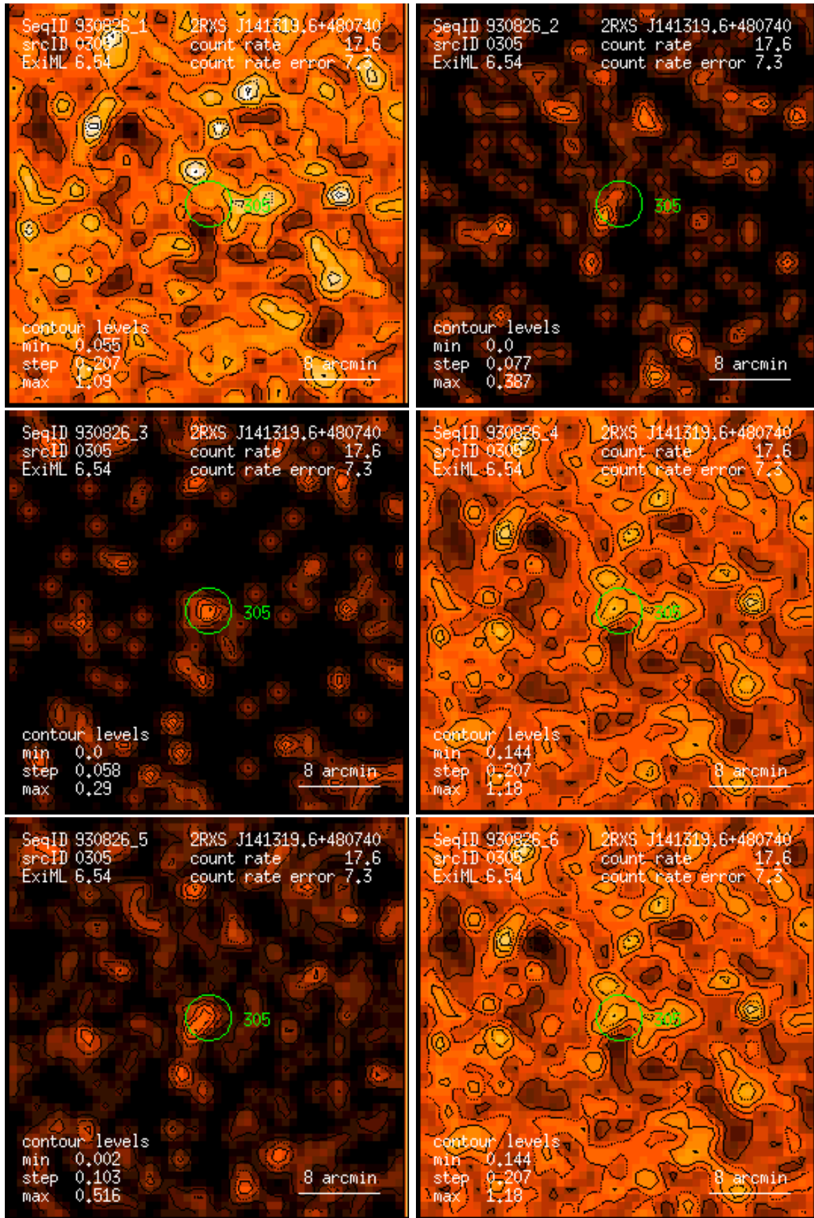
Figure 305: RASS 930826: detection 0305: band rate images, Gaussian filter: (1) PSPC channels 11 – 41, (2) 52 – 90, (3) 91 – 201, (4) 11 – 235, (5) 52 – 201, (6) 11 – 201. Broad band rates in counts/ks. Band rate contour levels in counts/ks/arcmin 2 .
