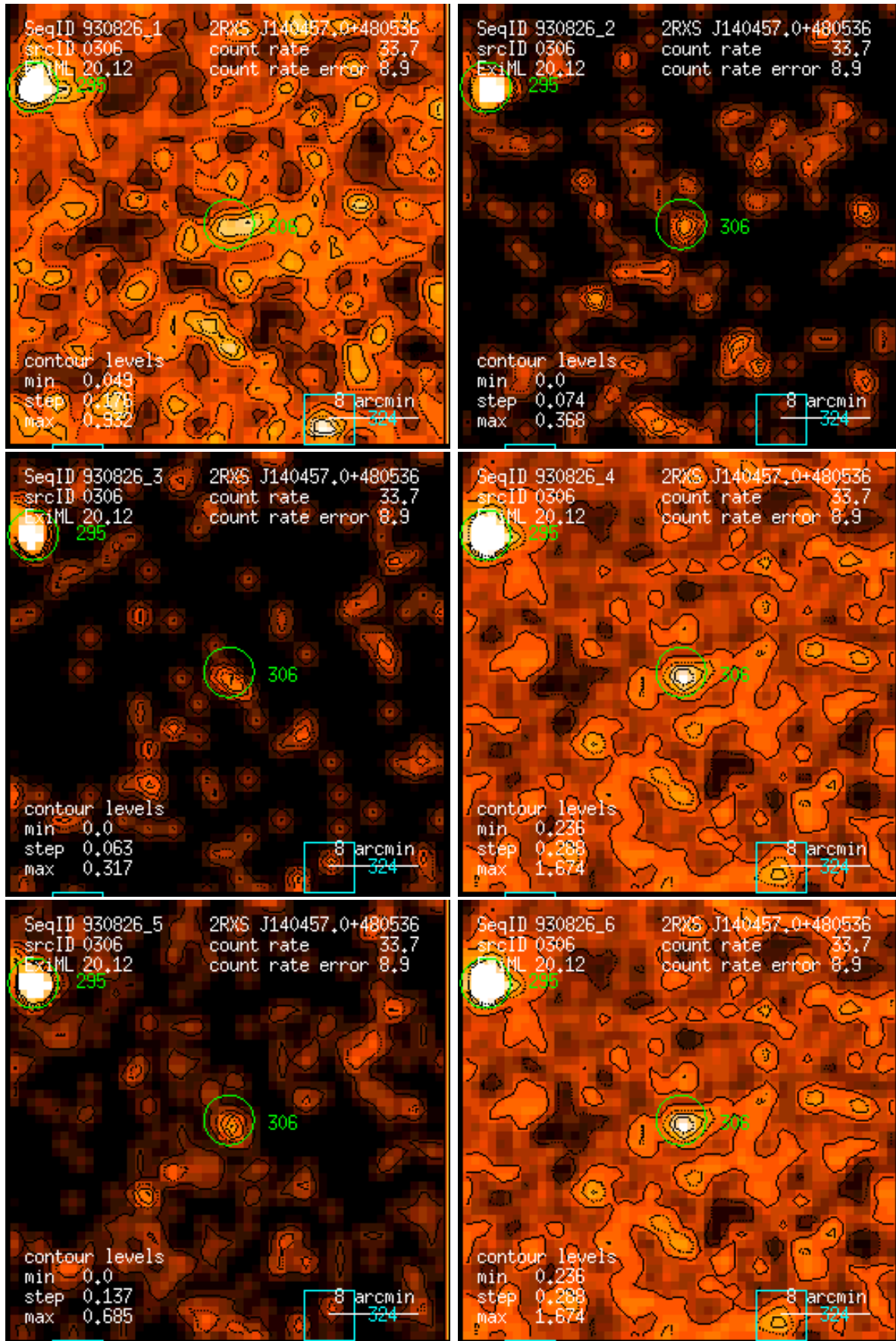
Figure 306: RASS 930826: detection 0306: band rate images, Gaussian filter: (1) PSPC channels 11 – 41, (2) 52 – 90, (3) 91 – 201, (4) 11 – 235, (5) 52 – 201, (6) 11 – 201. Broad band rates in counts/ks. Band rate contour levels in counts/ks/arcmin 2 .
