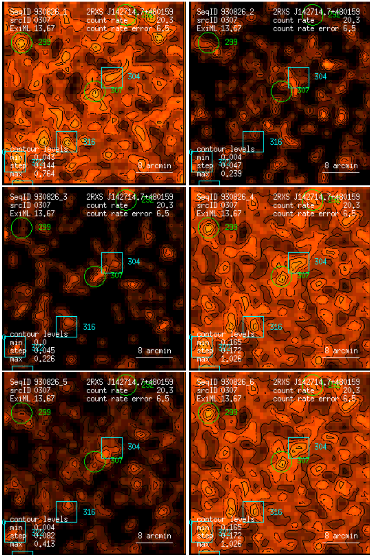
Figure 307: RASS 930826: detection 0307: band rate images, Gaussian filter: (1) PSPC channels 11 – 41, (2) 52 – 90, (3) 91 – 201, (4) 11 – 235, (5) 52 – 201, (6) 11 – 201. Broad band rates in counts/ks. Band rate contour levels in counts/ks/arcmin 2 .
