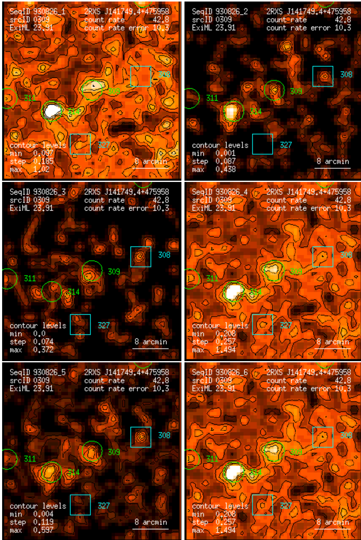
Figure 309: RASS 930826: detection 0309: band rate images, Gaussian filter: (1) PSPC channels 11 – 41, (2) 52 – 90, (3) 91 – 201, (4) 11 – 235, (5) 52 – 201, (6) 11 – 201. Broad band rates in counts/ks. Band rate contour levels in counts/ks/arcmin 2 .
