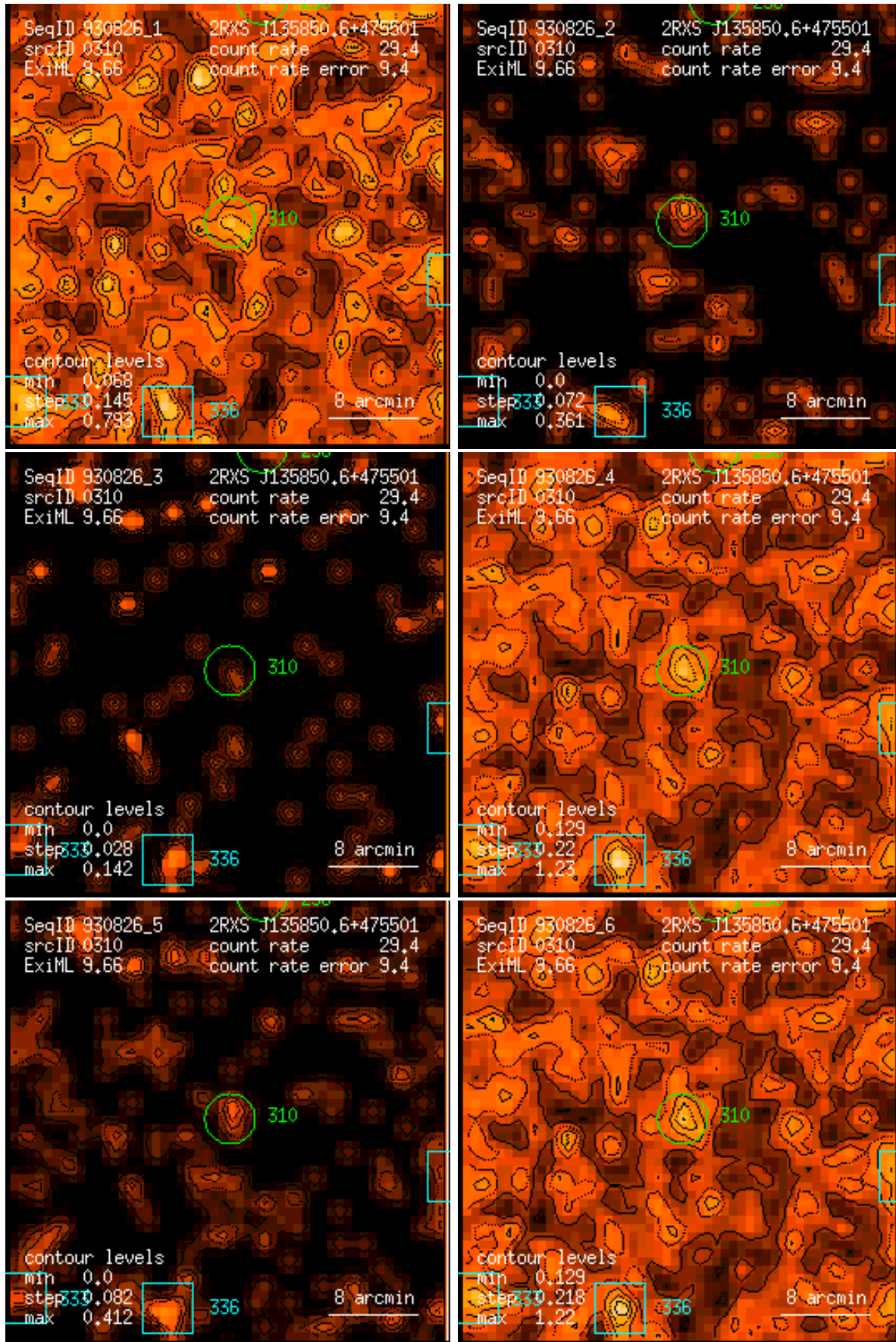
Figure 310: RASS 930826: detection 0310: band rate images, Gaussian filter: (1) PSPC channels 11 – 41, (2) 52 – 90, (3) 91 – 201, (4) 11 – 235, (5) 52 – 201, (6) 11 – 201. Broad band rates in counts/ks. Band rate contour levels in counts/ks/arcmin 2 .
