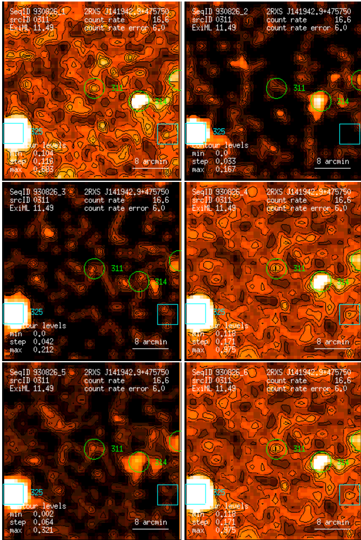
Figure 311: RASS 930826: detection 0311: band rate images, Gaussian filter: (1) PSPC channels 11 – 41, (2) 52 – 90, (3) 91 – 201, (4) 11 – 235, (5) 52 – 201, (6) 11 – 201. Broad band rates in counts/ks. Band rate contour levels in counts/ks/arcmin 2 .
