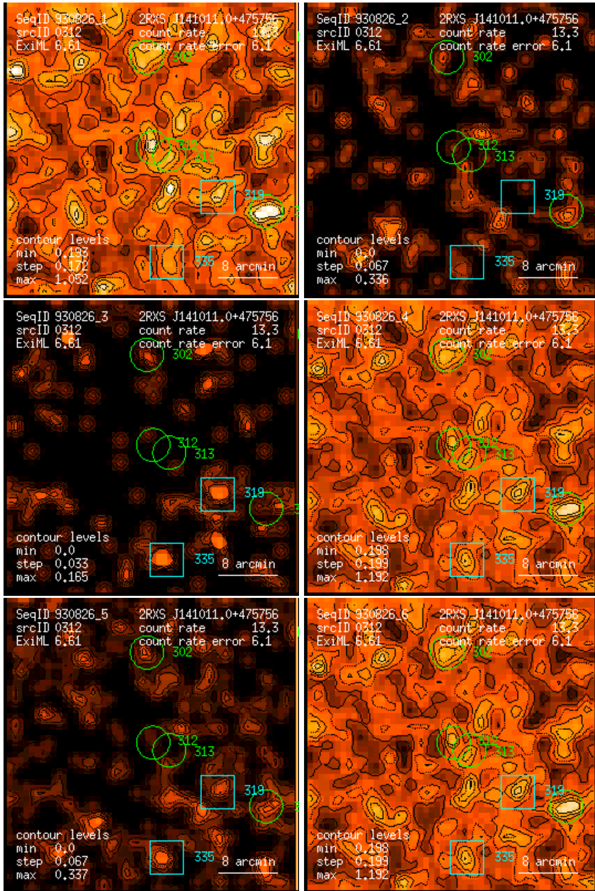
Figure 312: RASS 930826: detection 0312: band rate images, Gaussian filter: (1) PSPC channels 11 – 41, (2) 52 – 90, (3) 91 – 201, (4) 11 – 235, (5) 52 – 201, (6) 11 – 201. Broad band rates in counts/ks. Band rate contour levels in counts/ks/arcmin 2 .
