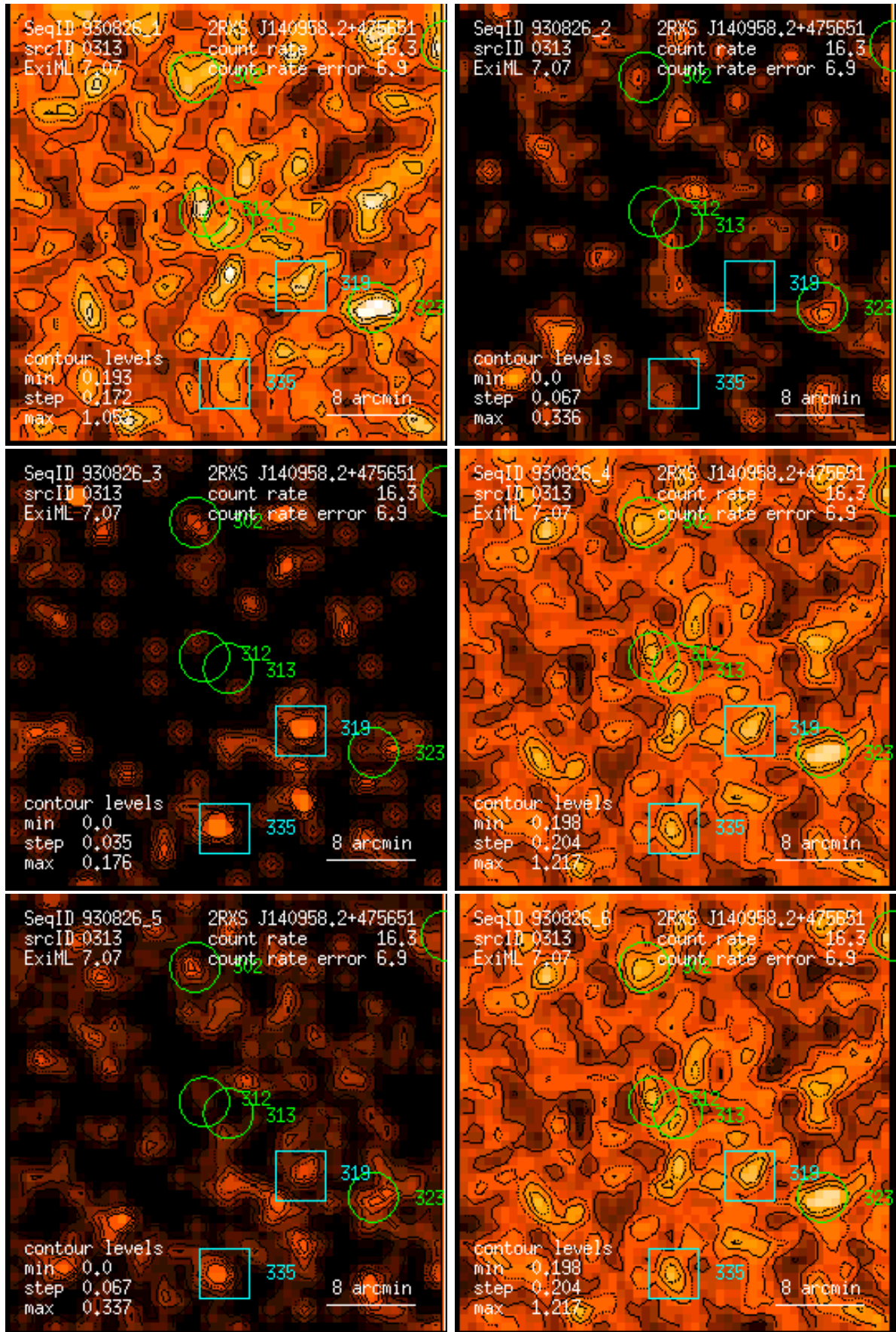
Figure 313: RASS 930826: detection 0313: band rate images, Gaussian filter: (1) PSPC channels 11 – 41, (2) 52 – 90, (3) 91 – 201, (4) 11 – 235, (5) 52 – 201, (6) 11 – 201. Broad band rates in counts/ks. Band rate contour levels in counts/ks/arcmin 2 .
