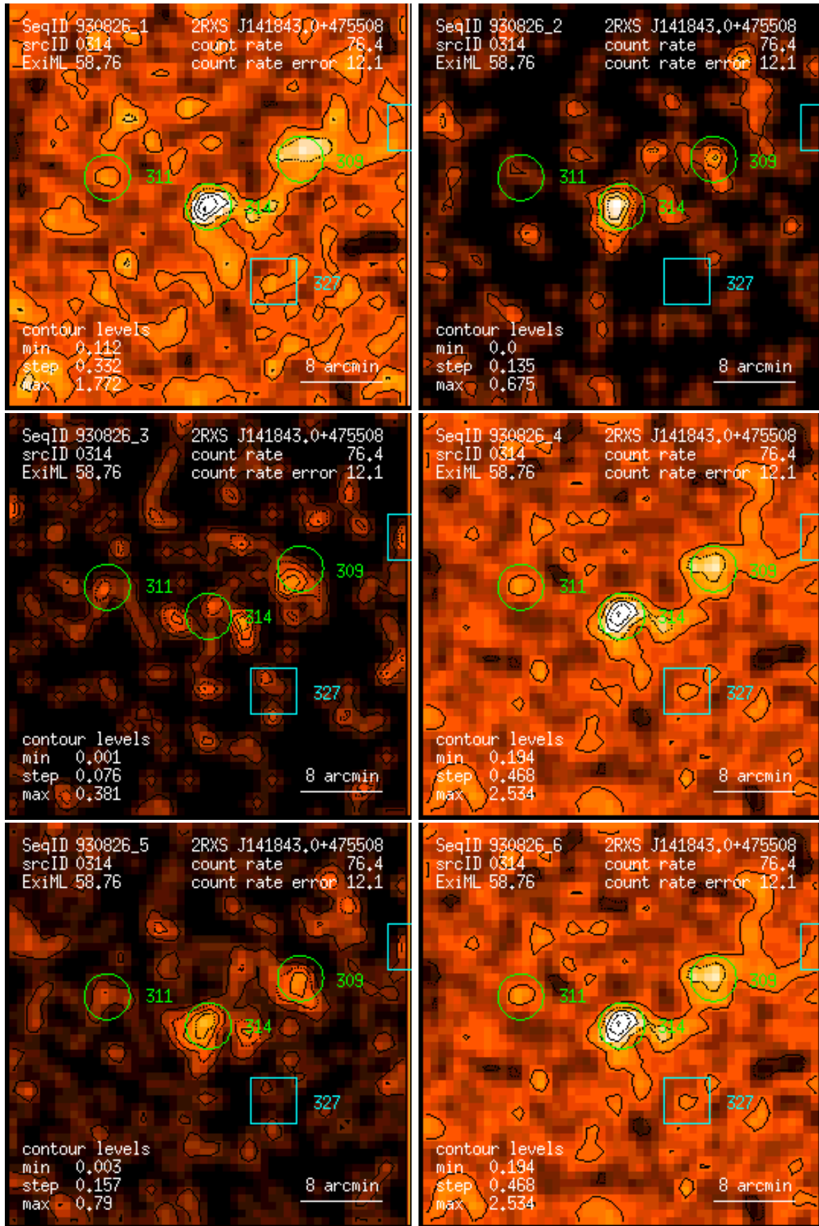
Figure 314: RASS 930826: detection 0314: band rate images, Gaussian filter: (1) PSPC channels 11 – 41, (2) 52 – 90, (3) 91 – 201, (4) 11 – 235, (5) 52 – 201, (6) 11 – 201. Broad band rates in counts/ks. Band rate contour levels in counts/ks/arcmin 2 .
