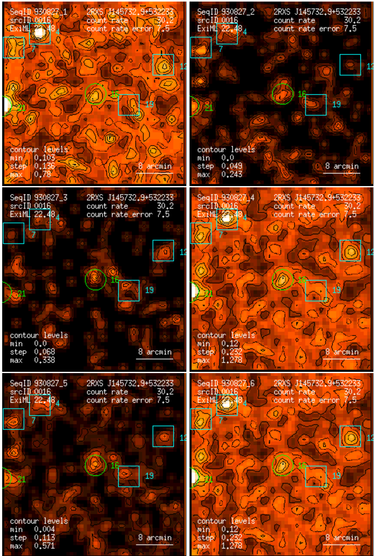
Figure 16: RASS 930827: detection 0016: band rate images, Gaussian filter: (1) PSPC channels 11 – 41, (2) 52 – 90, (3) 91 – 201, (4) 11 – 235, (5) 52 – 201, (6) 11 – 201. Broad band rates in counts/ks. Band rate contour levels in counts/ks/arcmin 2 .
