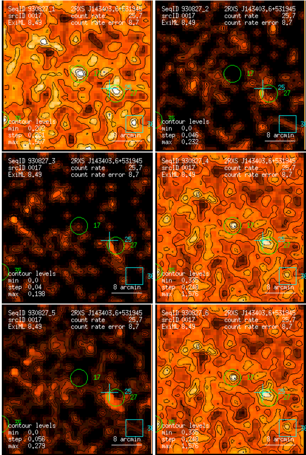
Figure 17: RASS 930827: detection 0017: band rate images, Gaussian filter: (1) PSPC channels 11 – 41, (2) 52 – 90, (3) 91 – 201, (4) 11 – 235, (5) 52 – 201, (6) 11 – 201. Broad band rates in counts/ks. Band rate contour levels in counts/ks/arcmin 2 .
