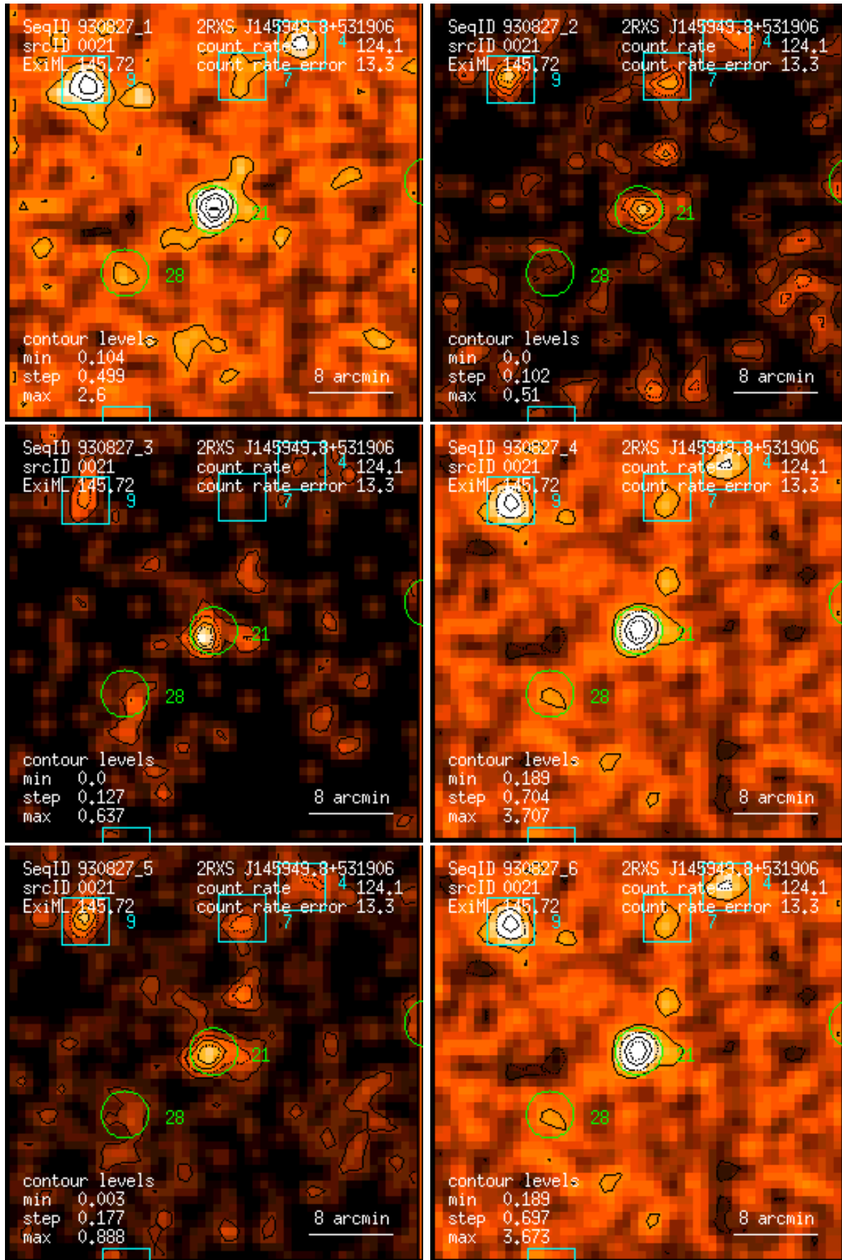
Figure 21: RASS 930827: detection 0021: band rate images, Gaussian filter: (1) PSPC channels 11 – 41, (2) 52 – 90, (3) 91 – 201, (4) 11 – 235, (5) 52 – 201, (6) 11 – 201. Broad band rates in counts/ks. Band rate contour levels in counts/ks/arcmin 2 .
