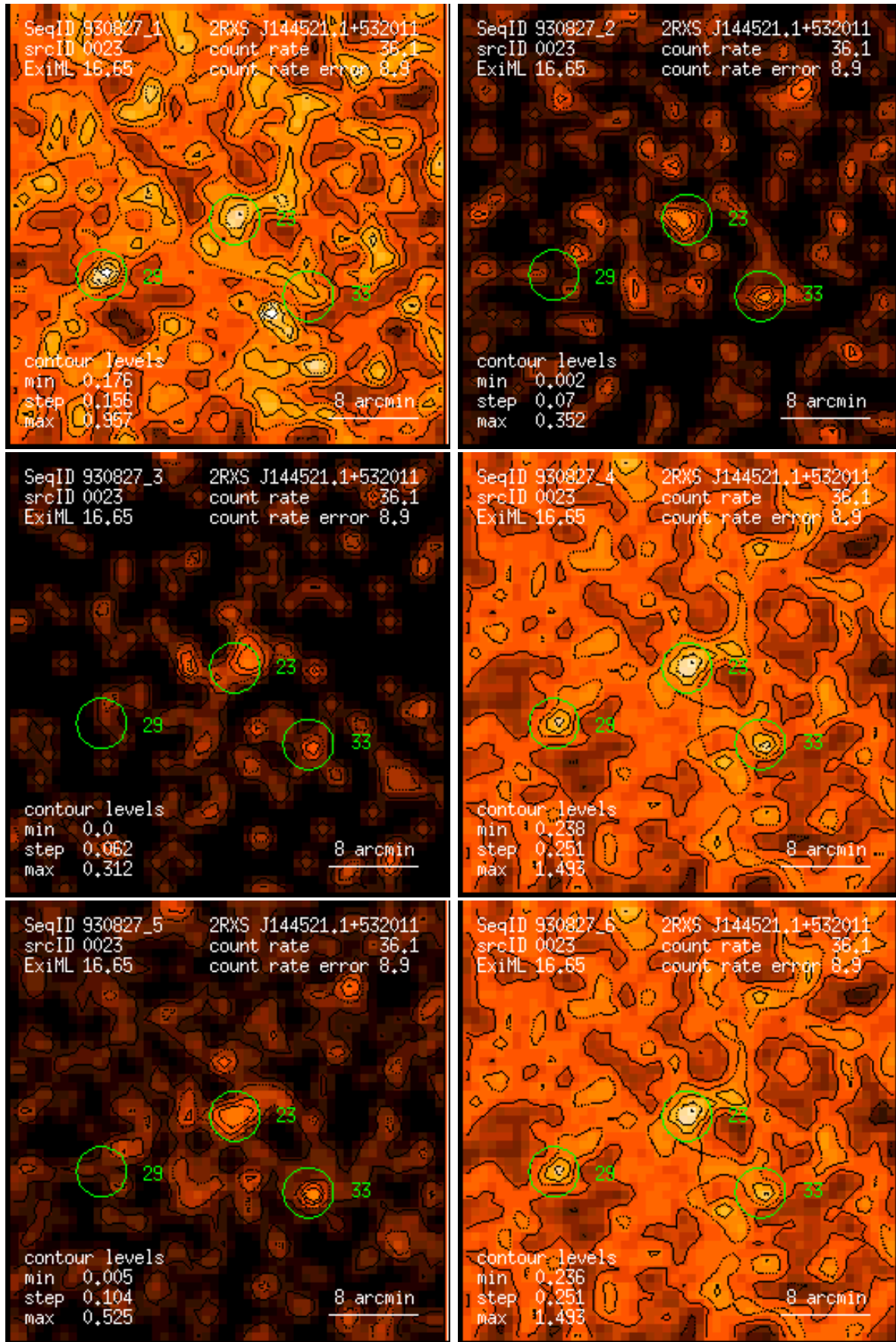
Figure 23: RASS 930827: detection 0023: band rate images, Gaussian filter: (1) PSPC channels 11 – 41, (2) 52 – 90, (3) 91 – 201, (4) 11 – 235, (5) 52 – 201, (6) 11 – 201. Broad band rates in counts/ks. Band rate contour levels in counts/ks/arcmin 2 .
