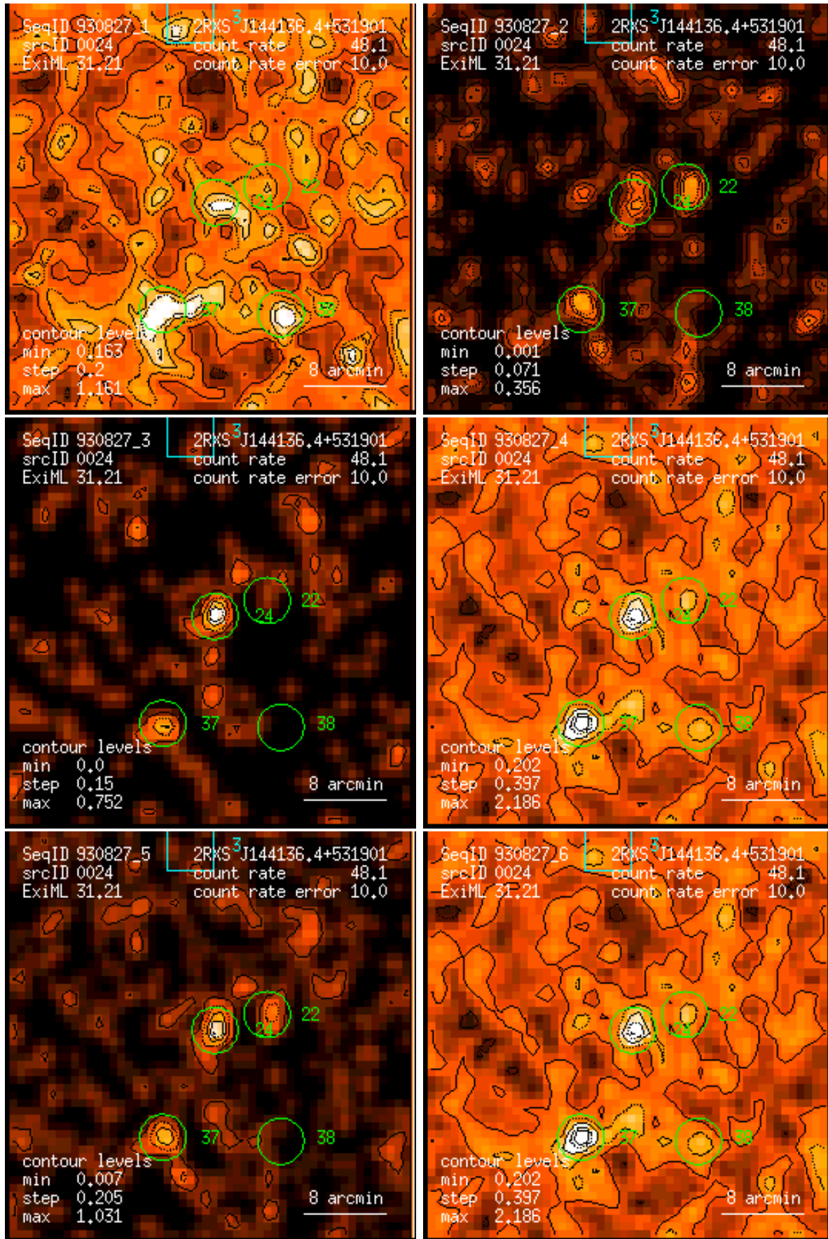
Figure 24: RASS 930827: detection 0024: band rate images, Gaussian filter: (1) PSPC channels 11 – 41, (2) 52 – 90, (3) 91 – 201, (4) 11 – 235, (5) 52 – 201, (6) 11 – 201. Broad band rates in counts/ks. Band rate contour levels in counts/ks/arcmin 2 .
