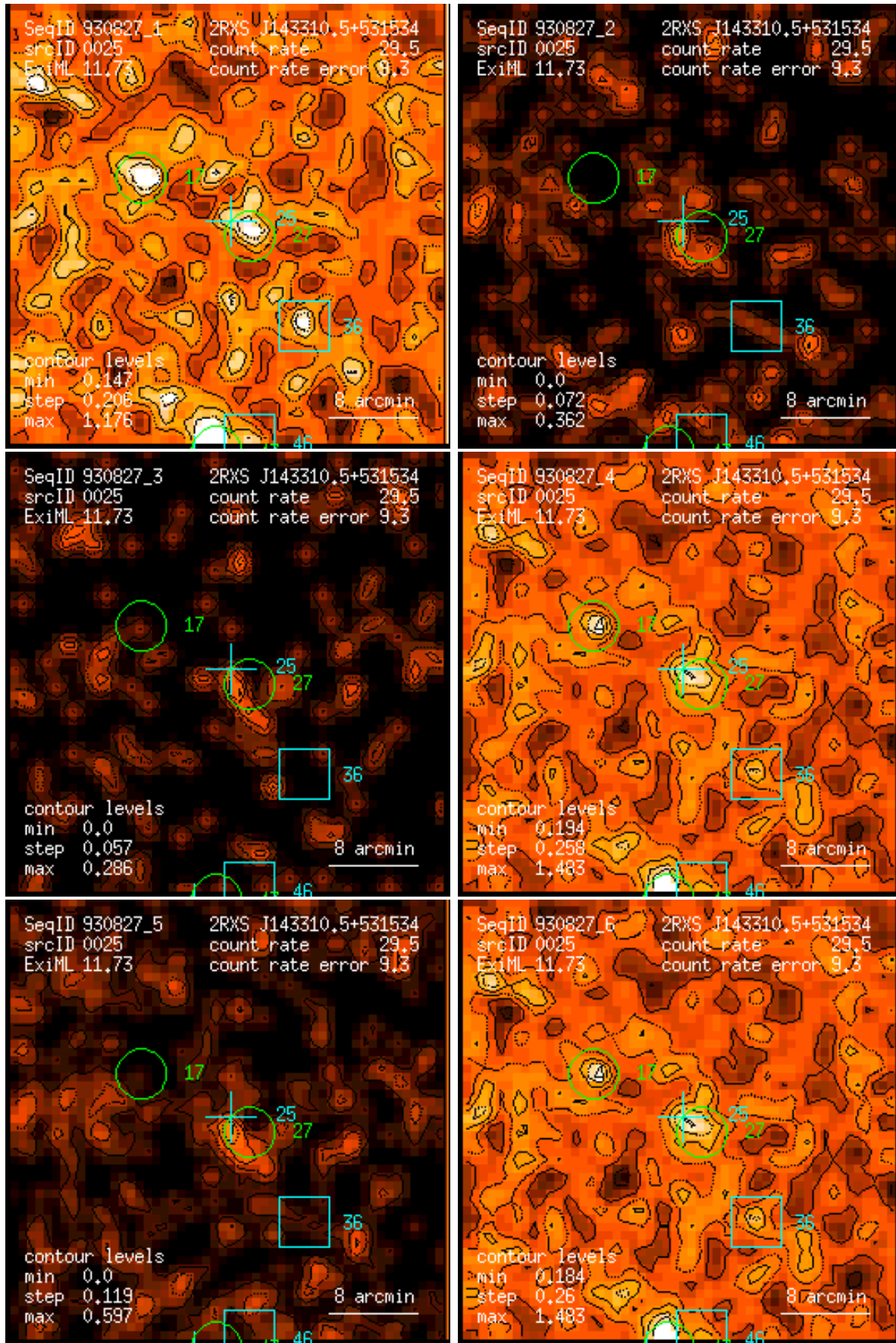
Figure 25: RASS 930827: detection 0025: band rate images, Gaussian filter: (1) PSPC channels 11 – 41, (2) 52 – 90, (3) 91 – 201, (4) 11 – 235, (5) 52 – 201, (6) 11 – 201. Broad band rates in counts/ks. Band rate contour levels in counts/ks/arcmin 2 .
