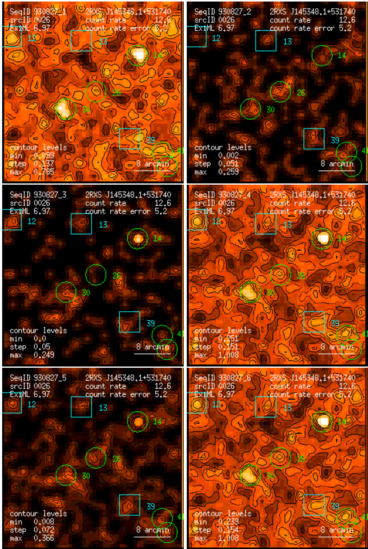
Figure 26: RASS 930827: detection 0026: band rate images, Gaussian filter: (1) PSPC channels 11 – 41, (2) 52 – 90, (3) 91 – 201, (4) 11 – 235, (5) 52 – 201, (6) 11 – 201. Broad band rates in counts/ks. Band rate contour levels in counts/ks/arcmin 2 .
