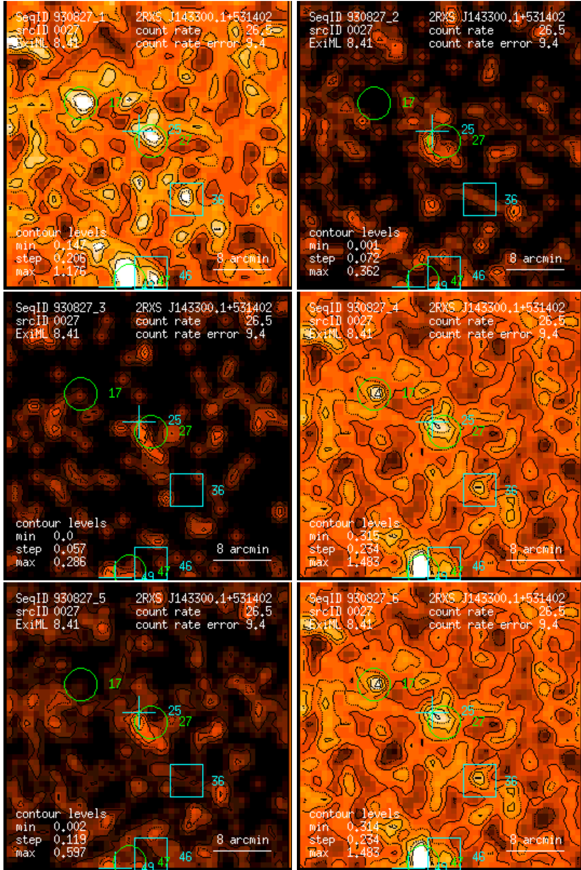
Figure 27: RASS 930827: detection 0027: band rate images, Gaussian filter: (1) PSPC channels 11 – 41, (2) 52 – 90, (3) 91 – 201, (4) 11 – 235, (5) 52 – 201, (6) 11 – 201. Broad band rates in counts/ks. Band rate contour levels in counts/ks/arcmin 2 .
