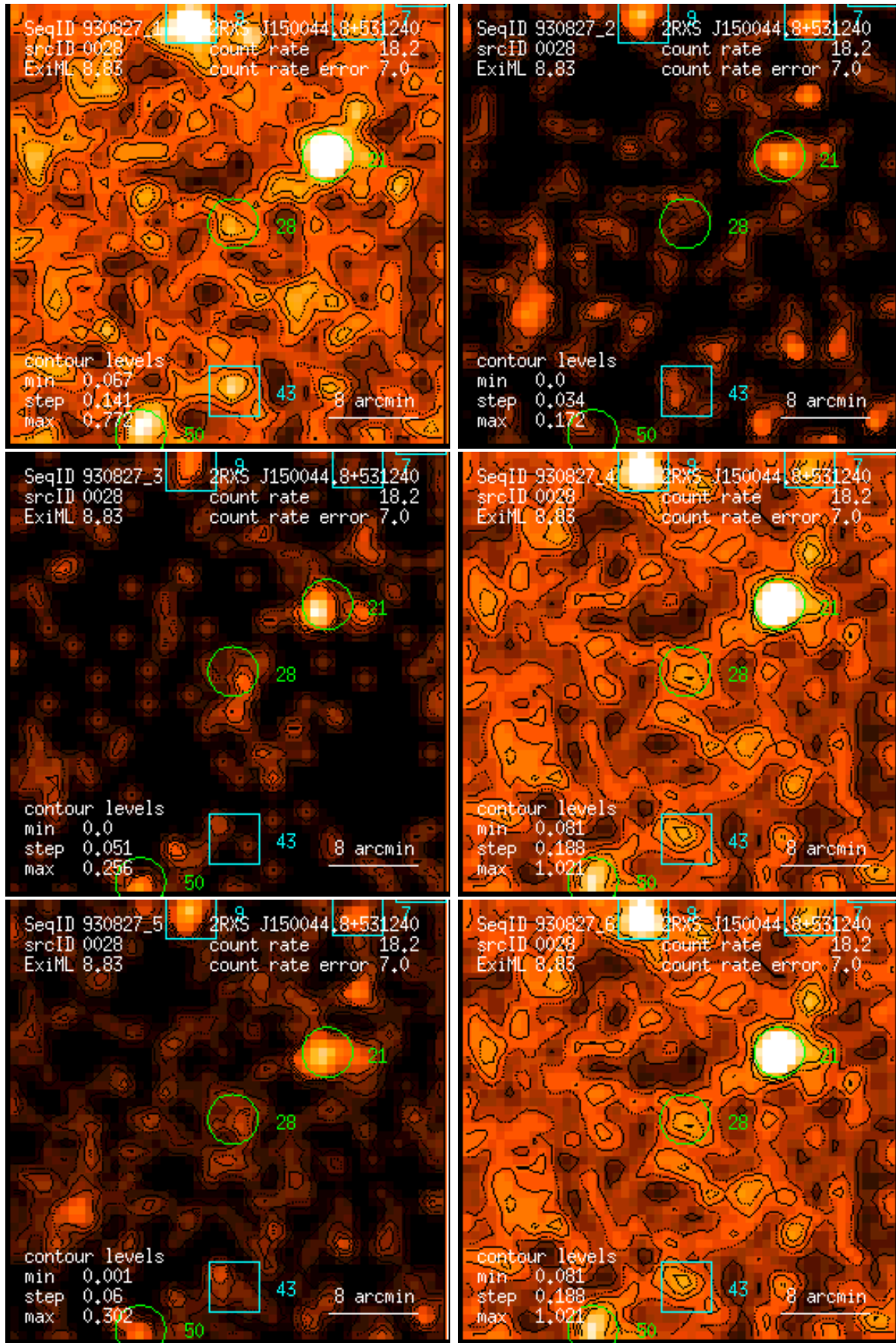
Figure 28: RASS 930827: detection 0028: band rate images, Gaussian filter: (1) PSPC channels 11 – 41, (2) 52 – 90, (3) 91 – 201, (4) 11 – 235, (5) 52 – 201, (6) 11 – 201. Broad band rates in counts/ks. Band rate contour levels in counts/ks/arcmin 2 .
