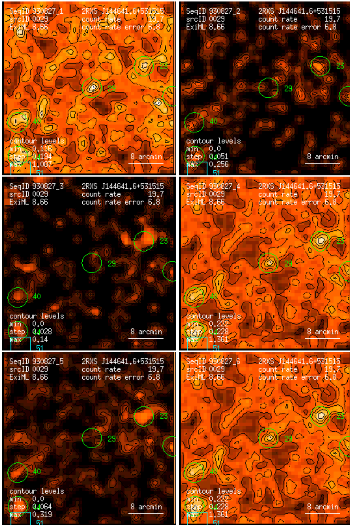
Figure 29: RASS 930827: detection 0029: band rate images, Gaussian filter: (1) PSPC channels 11 – 41, (2) 52 – 90, (3) 91 – 201, (4) 11 – 235, (5) 52 – 201, (6) 11 – 201. Broad band rates in counts/ks. Band rate contour levels in counts/ks/arcmin 2 .
