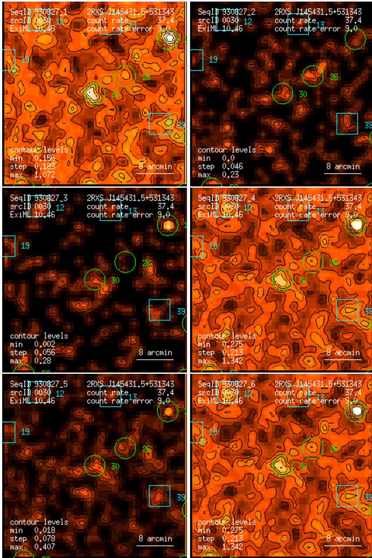
Figure 30: RASS 930827: detection 0030: band rate images, Gaussian filter: (1) PSPC channels 11 – 41, (2) 52 – 90, (3) 91 – 201, (4) 11 – 235, (5) 52 – 201, (6) 11 – 201. Broad band rates in counts/ks. Band rate contour levels in counts/ks/arcmin 2 .
