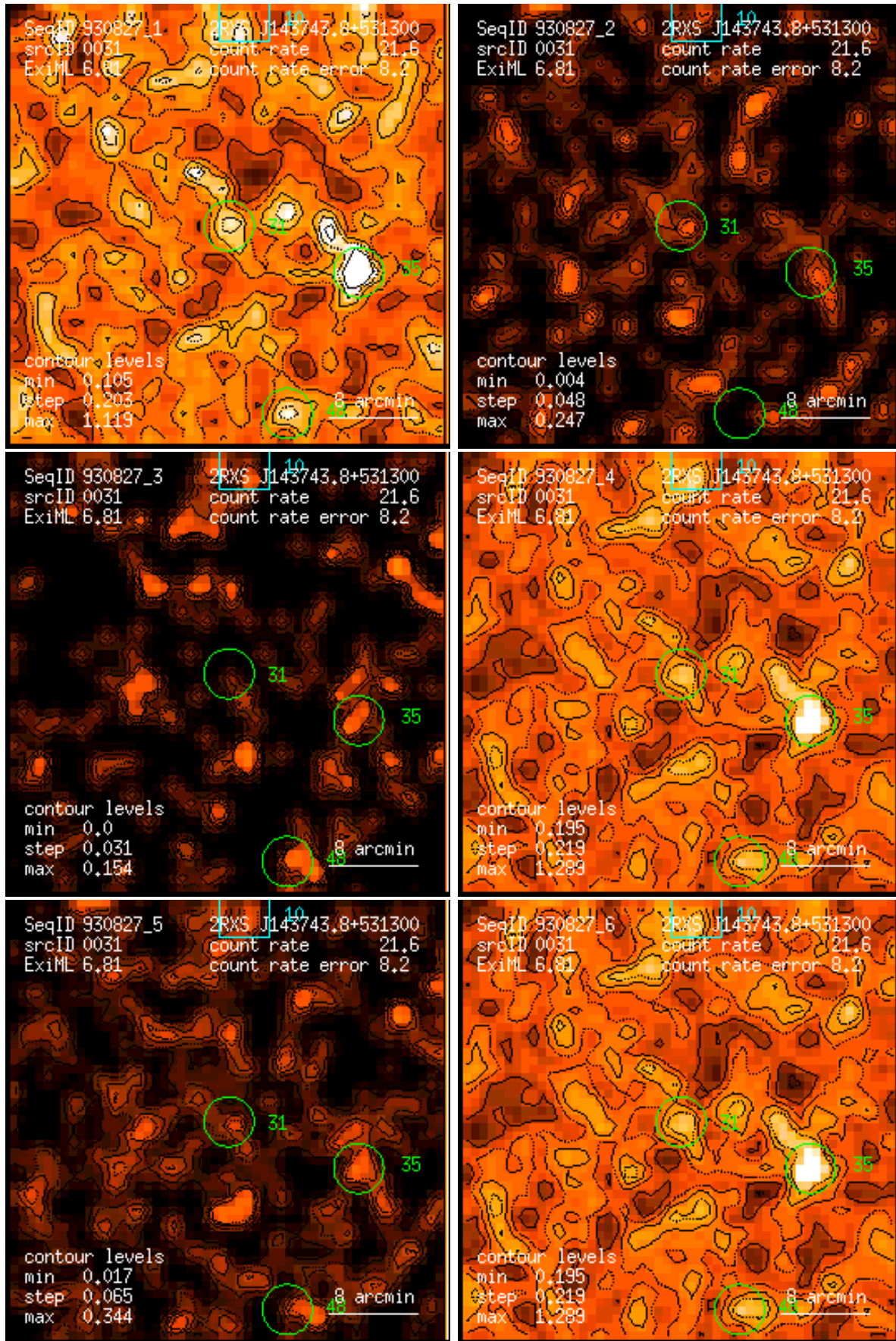
Figure 31: RASS 930827: detection 0031: band rate images, Gaussian filter: (1) PSPC channels 11 – 41, (2) 52 – 90, (3) 91 – 201, (4) 11 – 235, (5) 52 – 201, (6) 11 – 201. Broad band rates in counts/ks. Band rate contour levels in counts/ks/arcmin 2 .
