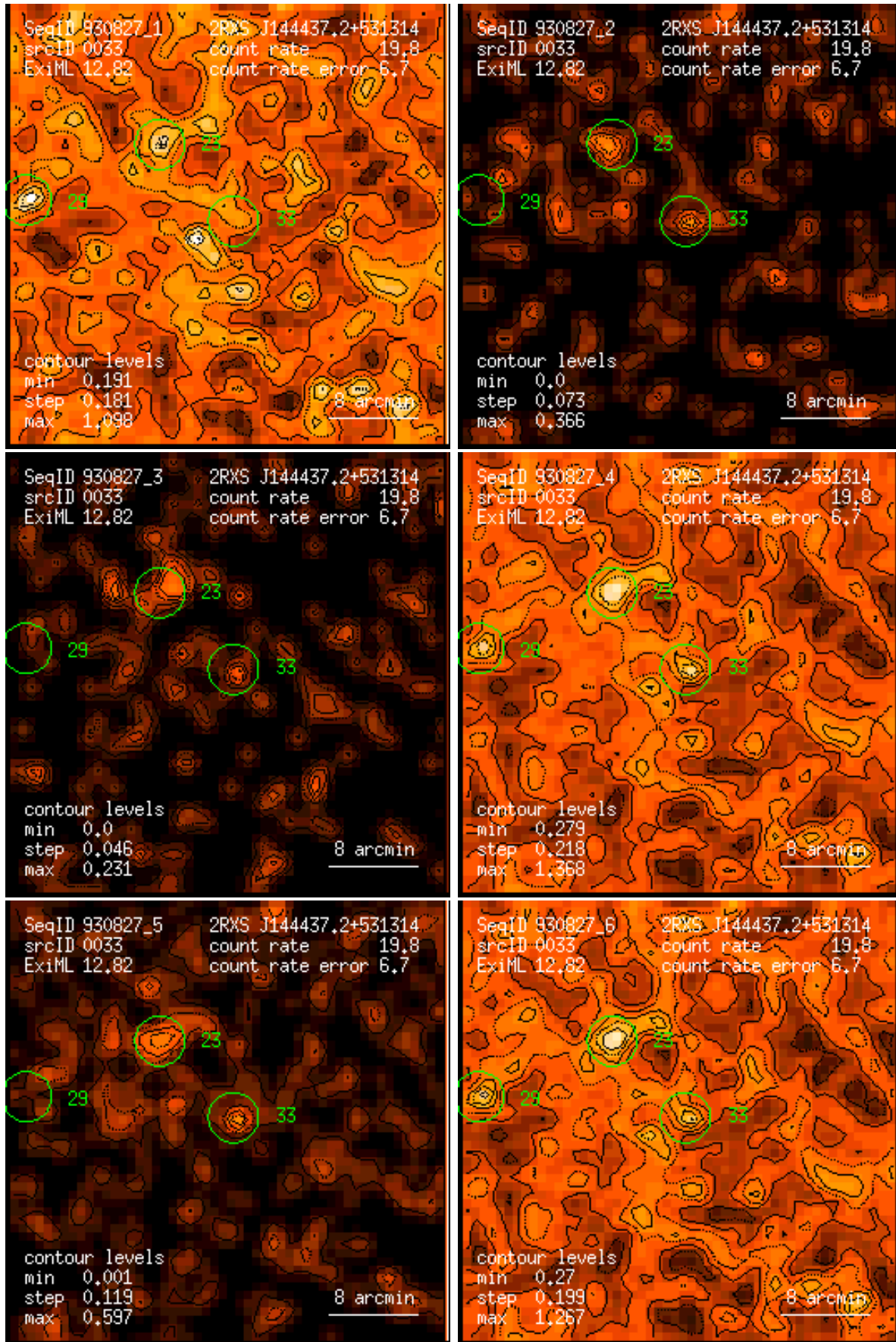
Figure 33: RASS 930827: detection 0033: band rate images, Gaussian filter: (1) PSPC channels 11 – 41, (2) 52 – 90, (3) 91 – 201, (4) 11 – 235, (5) 52 – 201, (6) 11 – 201. Broad band rates in counts/ks. Band rate contour levels in counts/ks/arcmin 2 .
